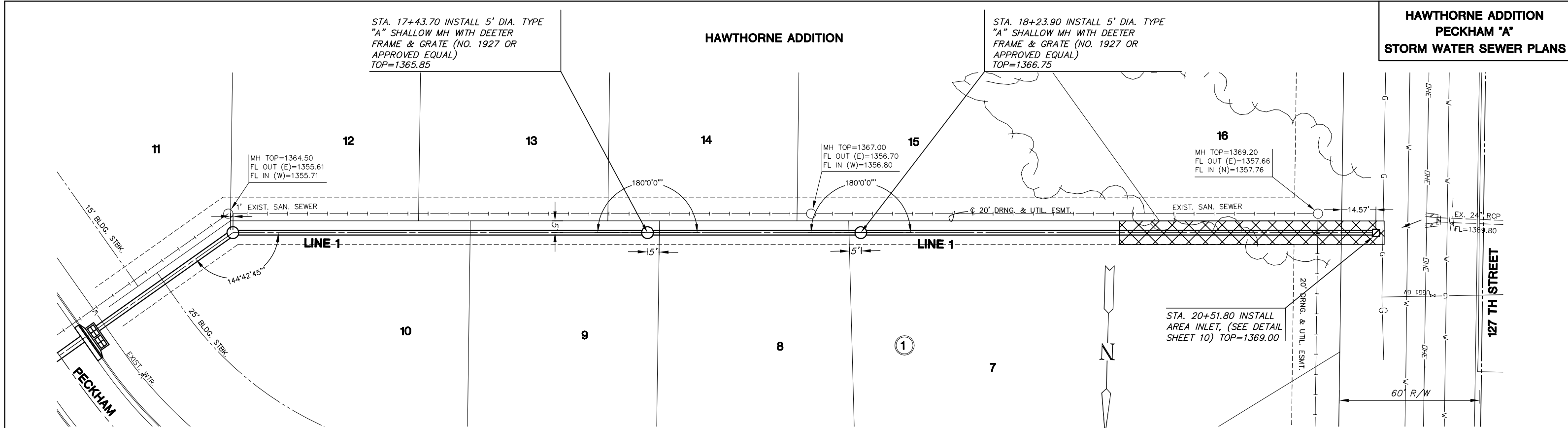
HAWTHORNE ADDITION PLAN LINE 1 CONT'D
