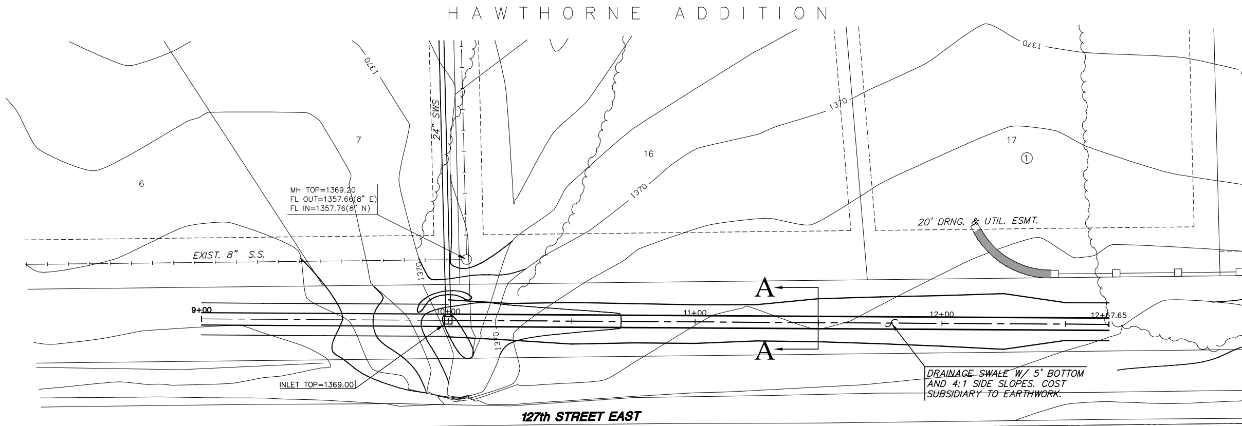
DITCH 1 PLAN SCALE: 1"=20'
