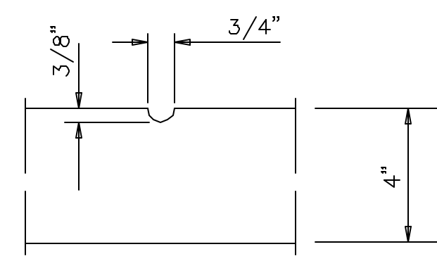
GROOVE DETAIL
