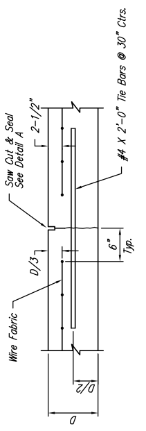
LONGITUDINAL JOINT DETAIL (L.J.)
