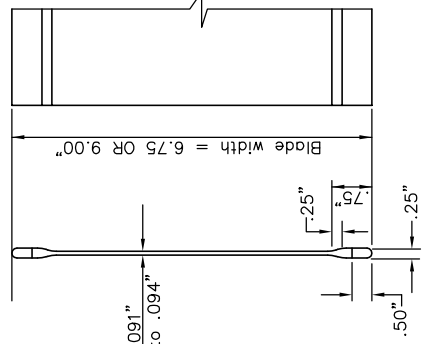
STREET NAME SIGN BLADE DETAILS
