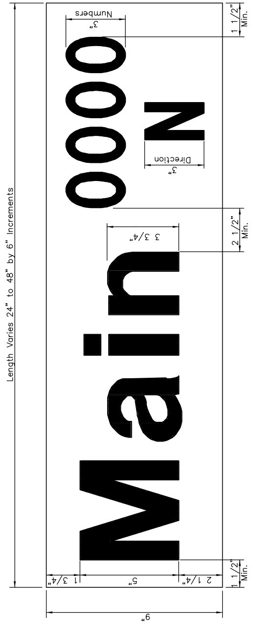
DETAIL B 9" METRO
