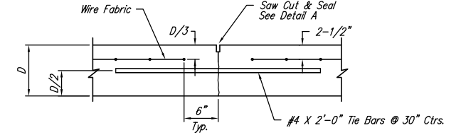
LONGITUDINAL JOINT DETAIL (L.J.)
