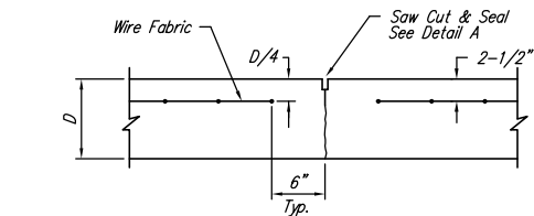
CONTRACTION JOINT DETAIL (C.J.)
