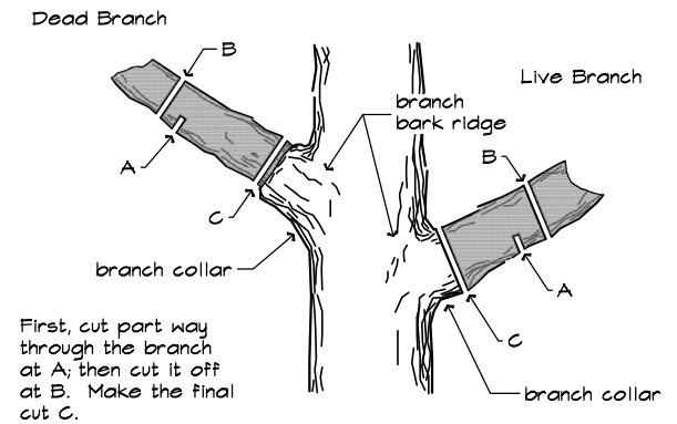
TREE TRIMMING DETAIL NOT TO SCALE
