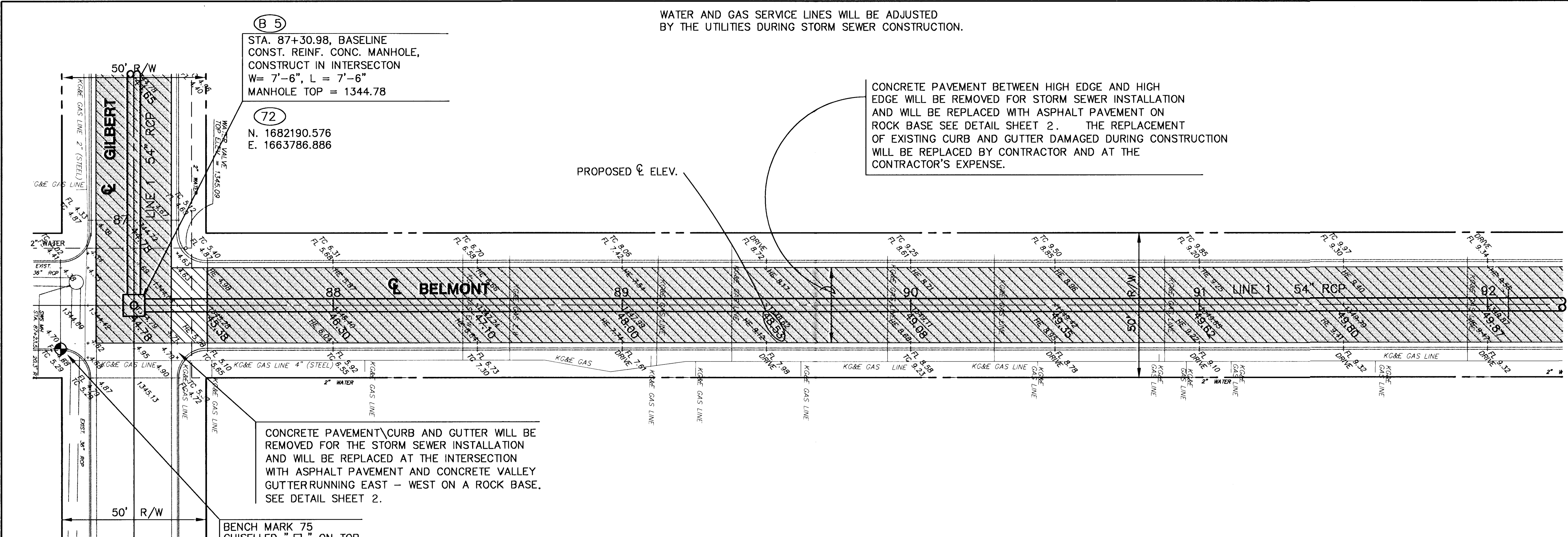
PLAN LINE 1
