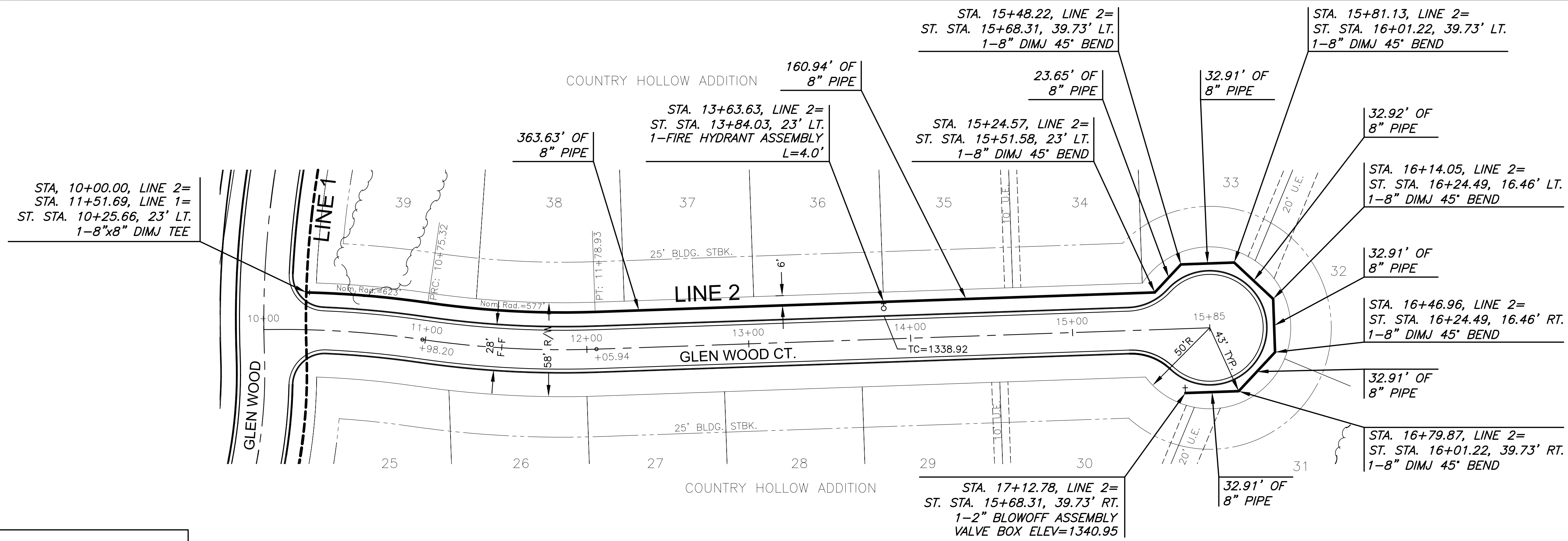
PLAN LINE 2 PROFILE LINE 2
