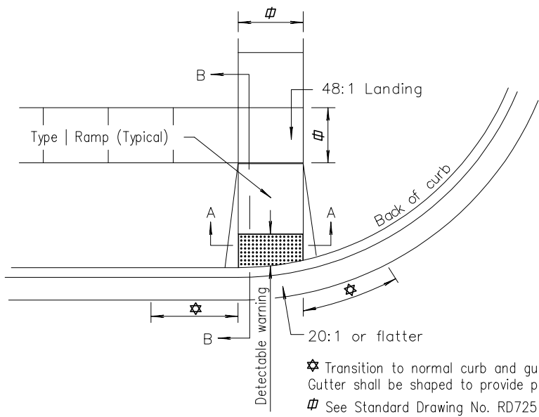
TYPICAL PLAN
