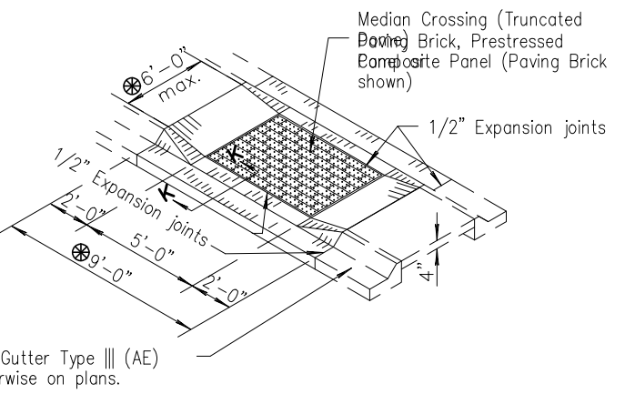
NARROW MEDIAN RAMP CROSSING
