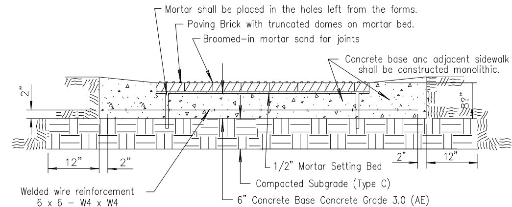
TYPICAL SECTION OF PAVER BRICK SECTION A-A
