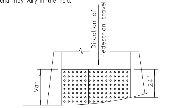
RADIUS CURB DETAILS (COMPOSITE) Cut Radius from 3'-0" Long Composite Panel.
