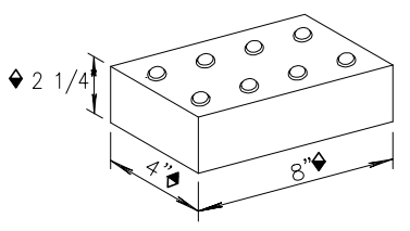
PAVER BRICK WITH TRUNCATED DOME SURFACE
