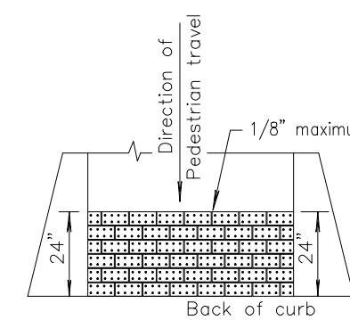
STRAIGHT CURB DETAILS
