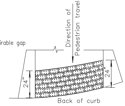
RADIUS CURB DETAILS
