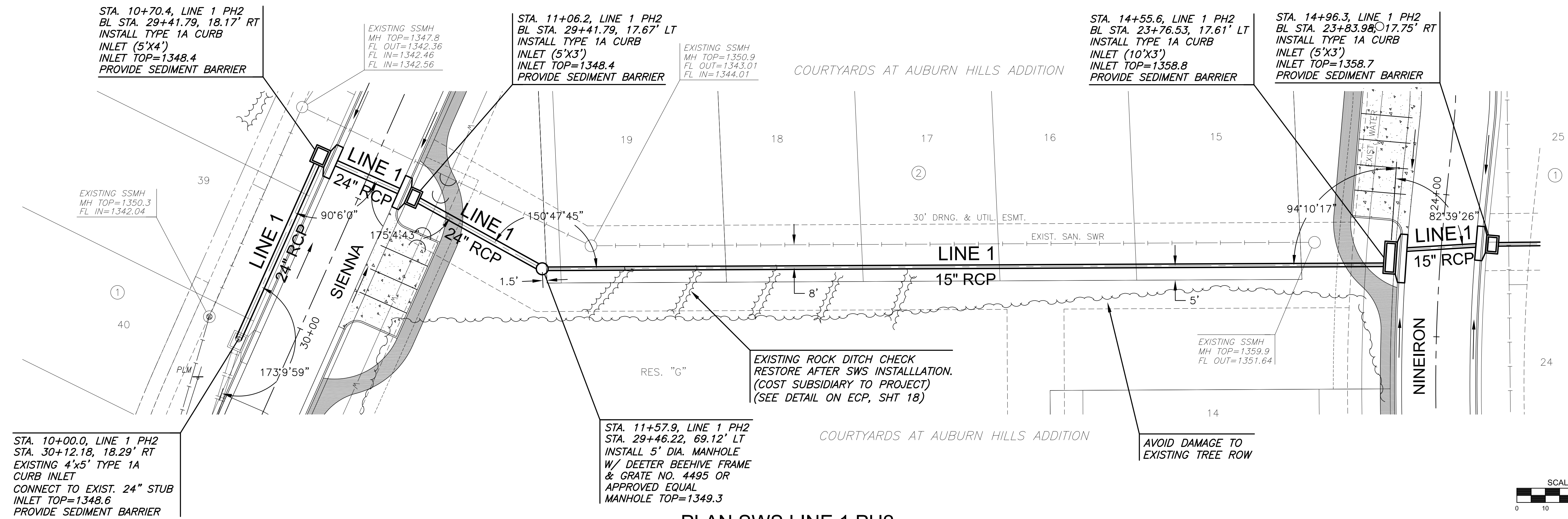
PLAN SWS LINE 1 PH2 PROFILE SWS LINE 1 PH2
