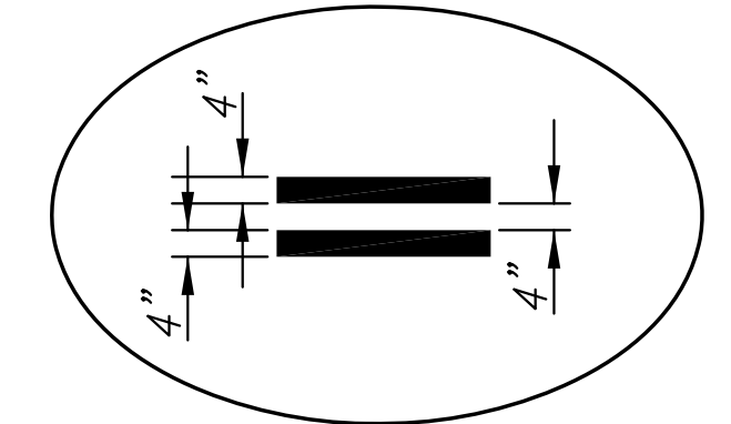
TYPICAL SPACING FOR 4" DOUBLE YELLOW LINE
