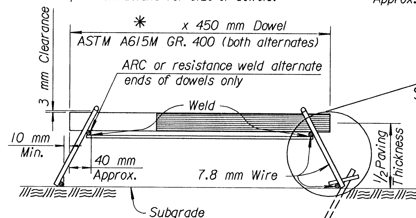
SEC. B-B
