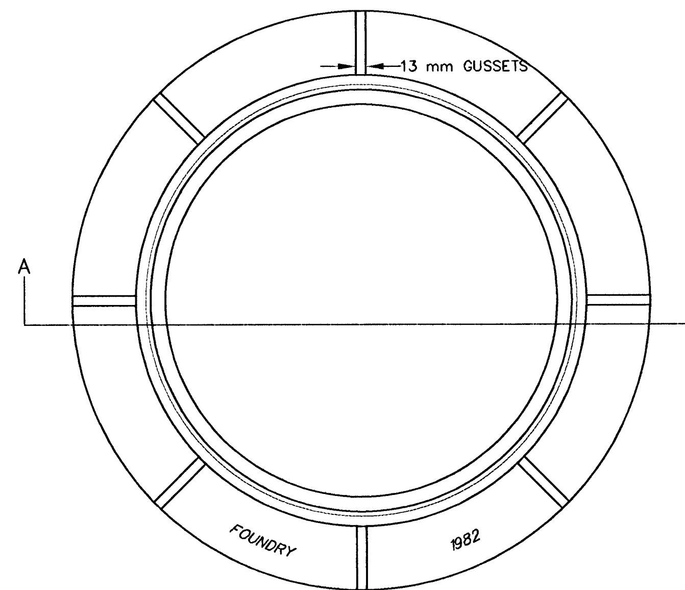
TOP VIEW
