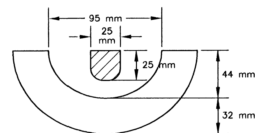
SECTION VIEW
