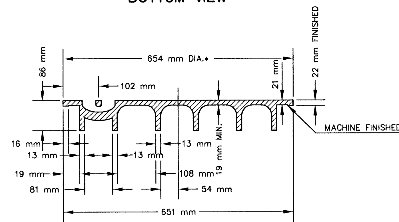
SECTION VIEW
