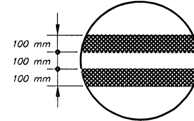
100 mm DOUBLE YELLOW DETAIL
