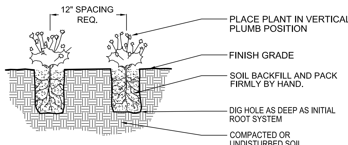
TYPICAL PLUG INSTALLATION NOT TO SCALE
