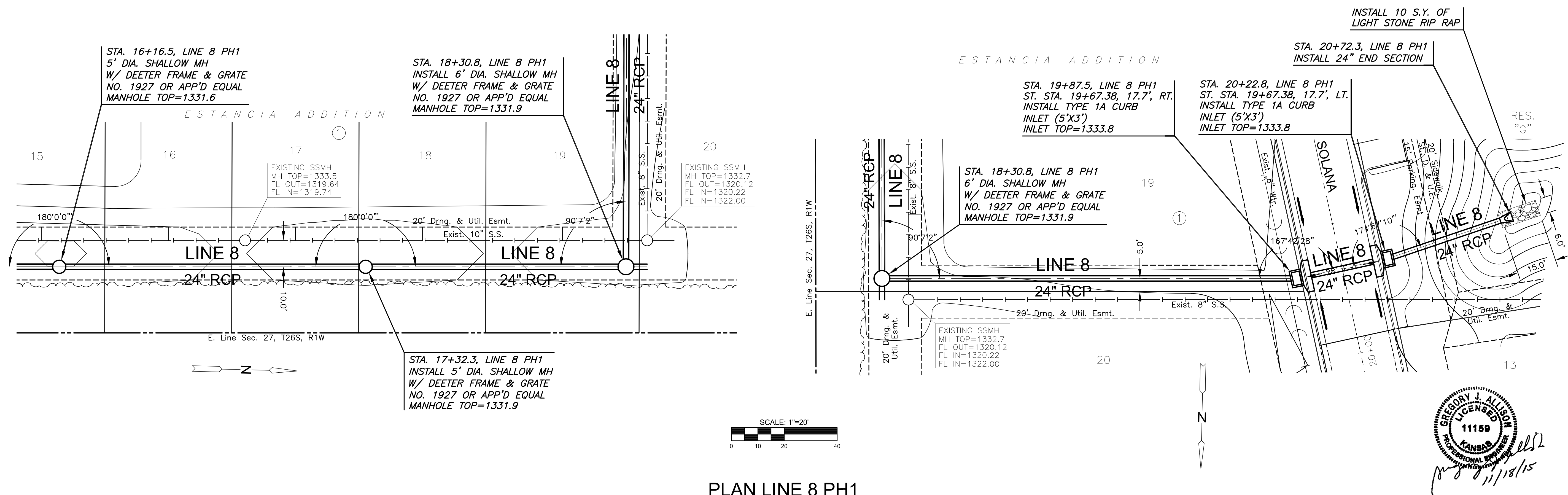
PLAN LINE 8 PH1 PROFILE LINE 8 PH1
