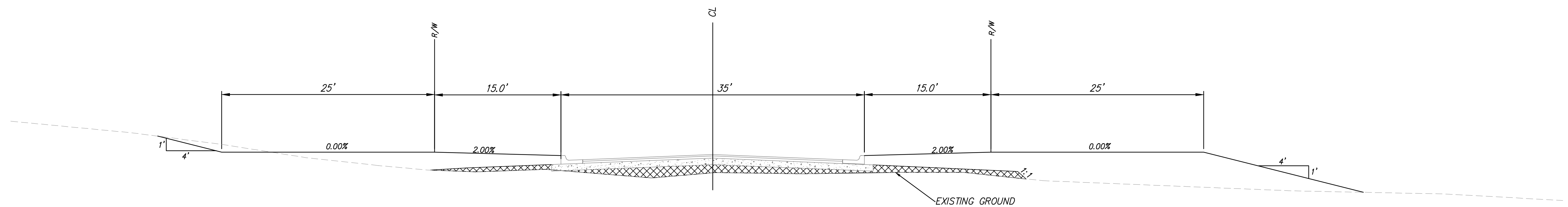
TYPICAL 64' ROW GRADING SECTION
