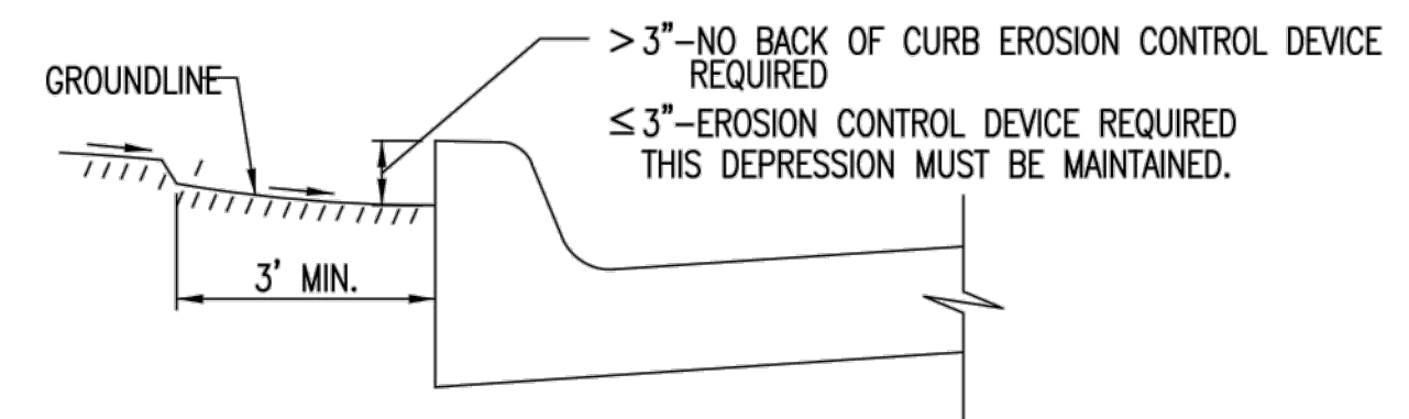
CURB BACKFILL DETAIL THIS IS A TEMPORARY MEASURE ONLY, WHEN APPROVED BY THE PROJECT ENGINEER. THE DIRT GRADE BEHIND THE CURB SHALL BE BROUGHT TO THE TOP OF CURB, WITH TEMPORARY EROSION CONTROL MAT OR PERMANENT VEGETATION PLACED, PRIOR TO THE COMPLETION OF ALL PROJECTS.
