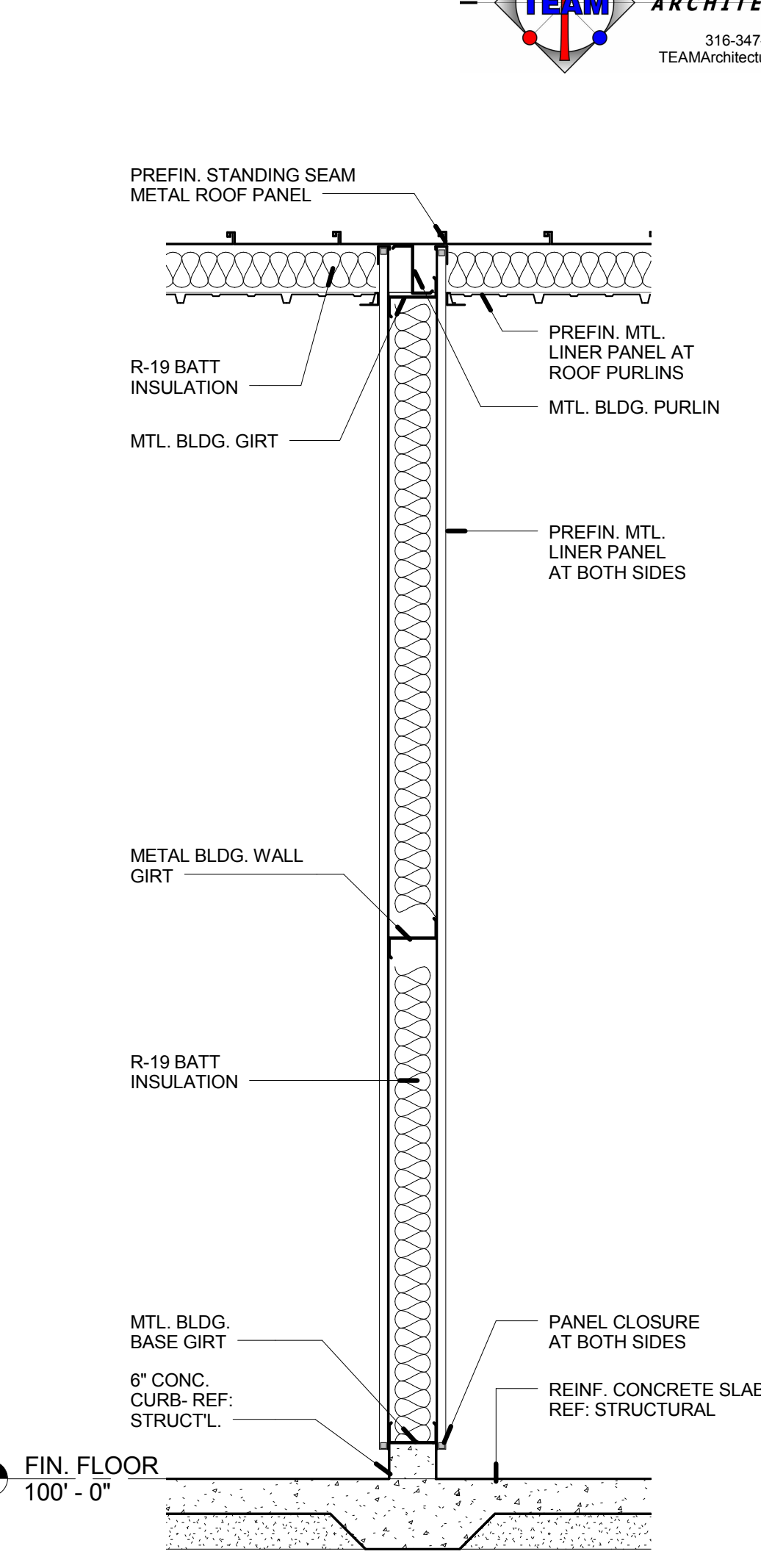
E MCC WALL 1/2" = 1'-0"
