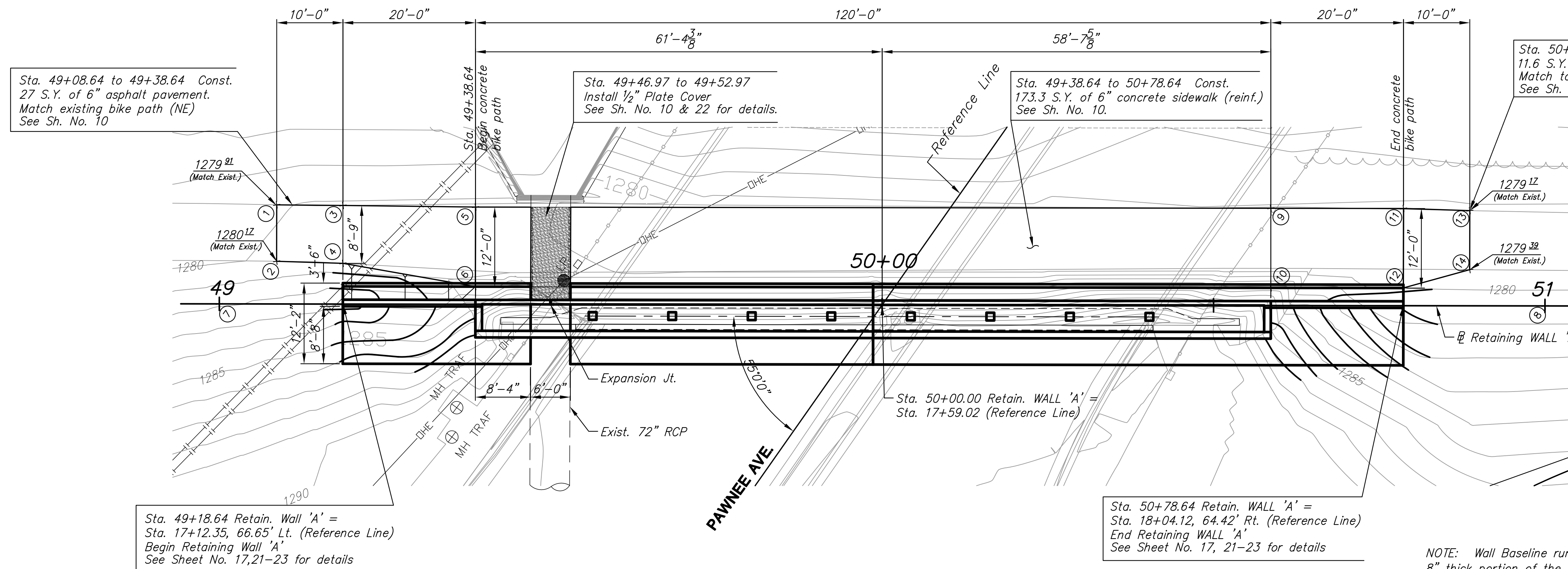
PLAN - RETAINING WALL 'A' WEST ABUTMENT
