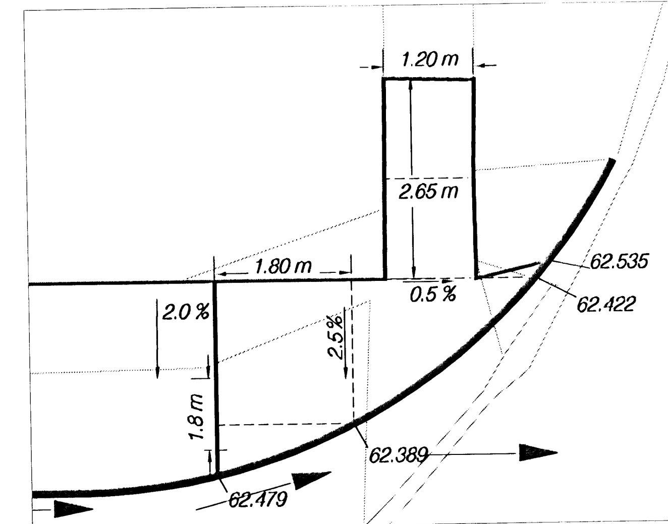
Wheelchair Ramp Detail, Sta. 3+182.320 Not On This Sheet, See Sheet 6
