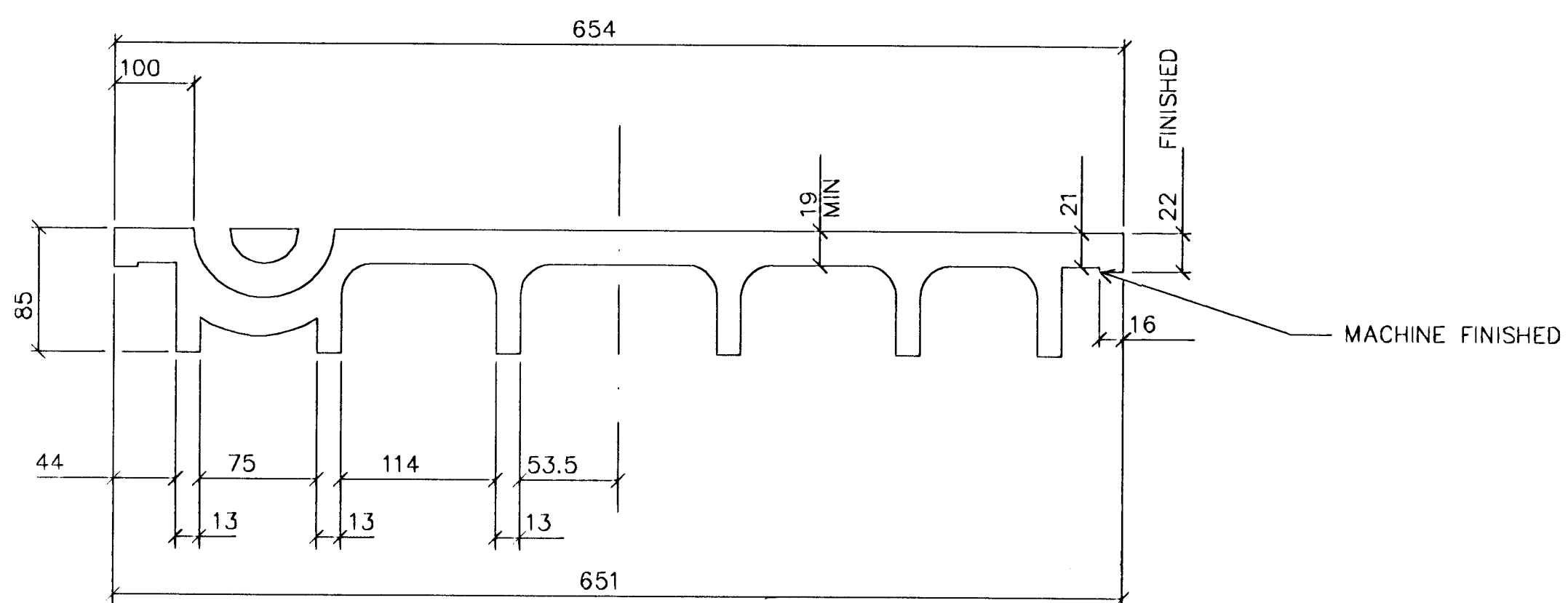
BOTTOM VIEW
