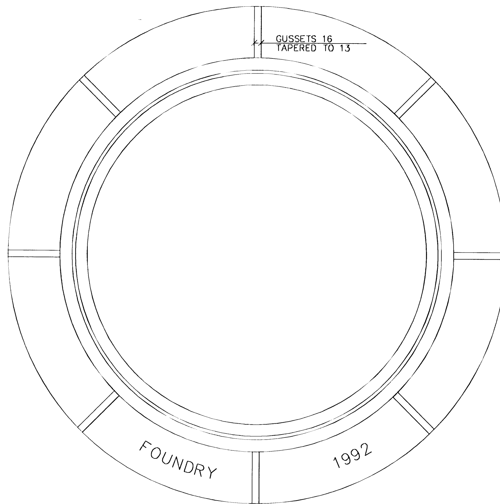
TOP VIEW
