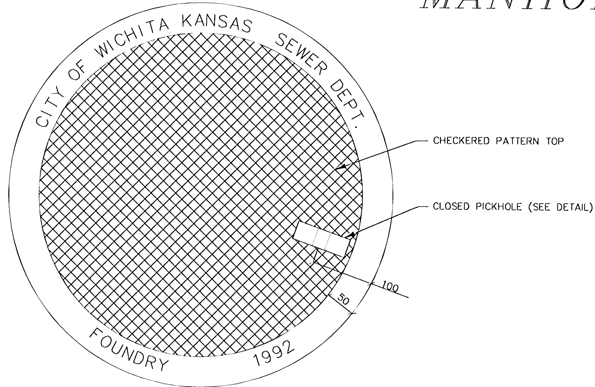
TOP VIEW
