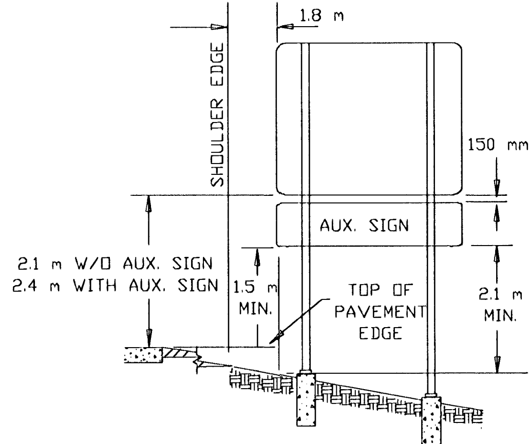
SHOULDER INSTALLED SIGN WITH OR WITHOUT AUX. SIGN
