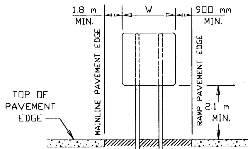
GORE INSTALLED SIGN (BETWEEN MAINLINE AND RAMP)
