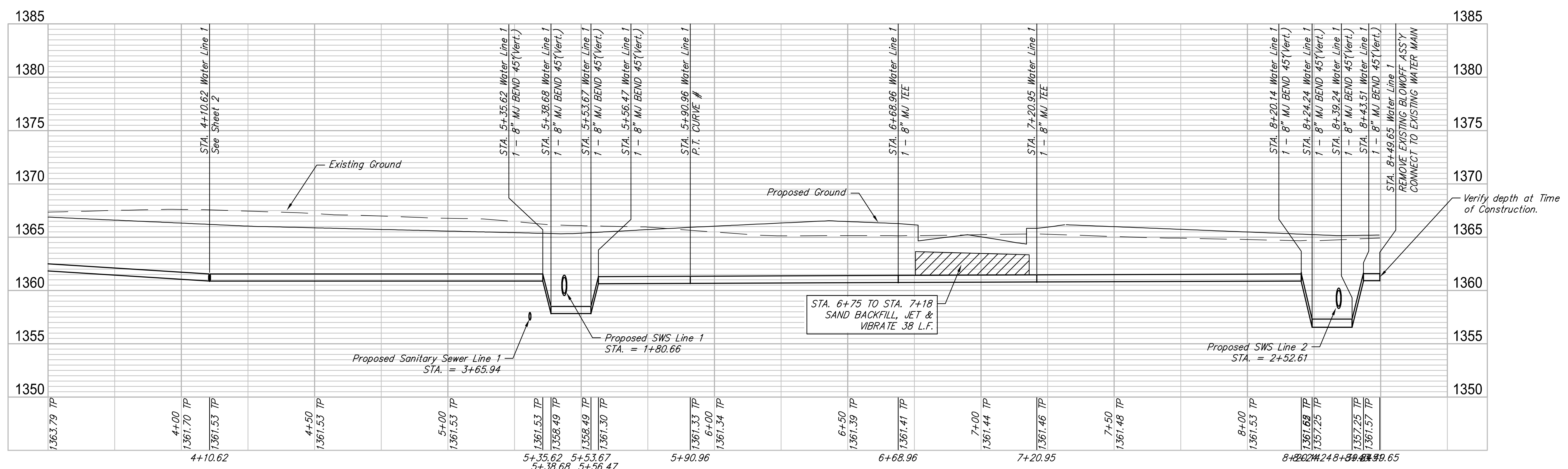
Water Line 1 PROFILE
