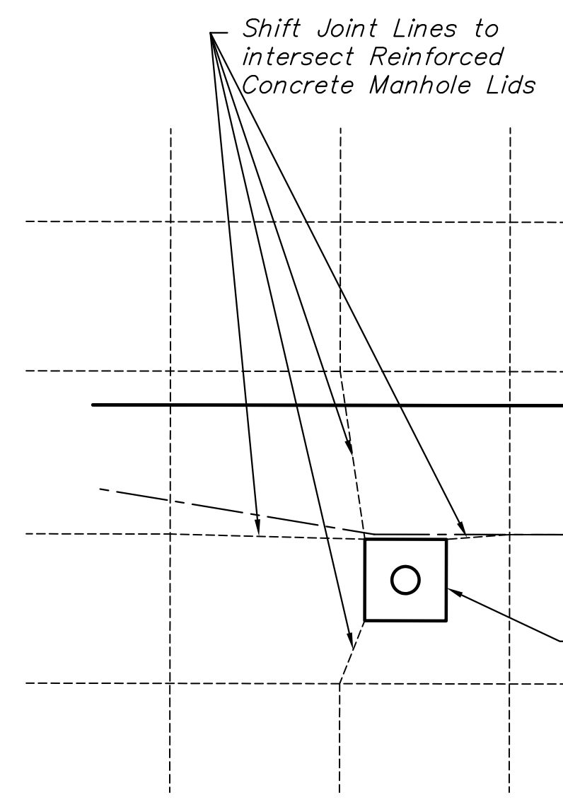
CONCRETE JOINTING AT REINFORCED CONCRETE MANHOLE LIDS
