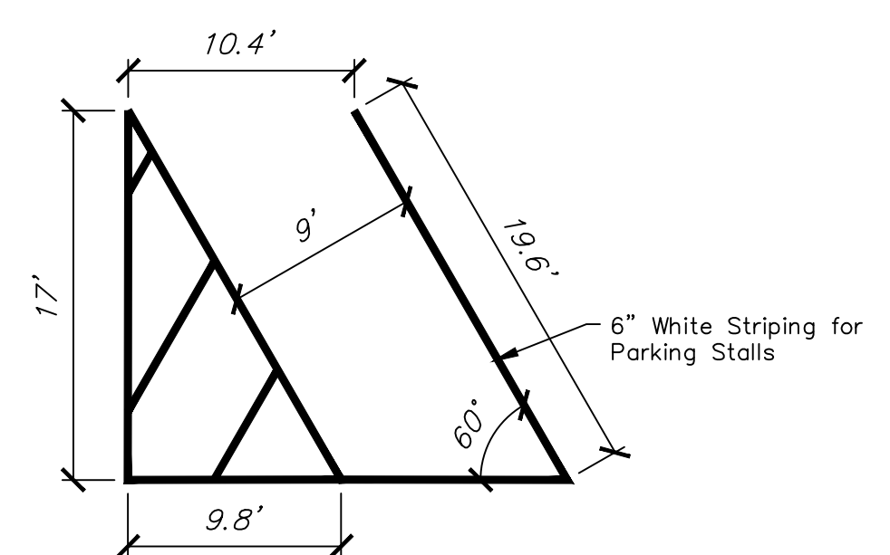
1 TYP. ANGLED PARKING STALL NOT TO SCALE
