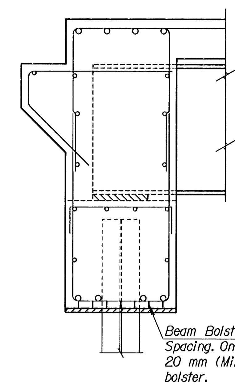
ABUTMENT
