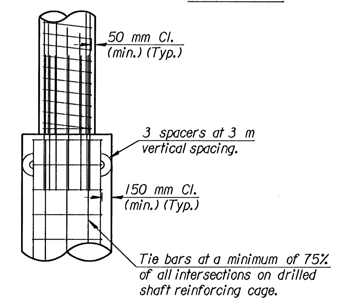
DRILLED SHAFT
