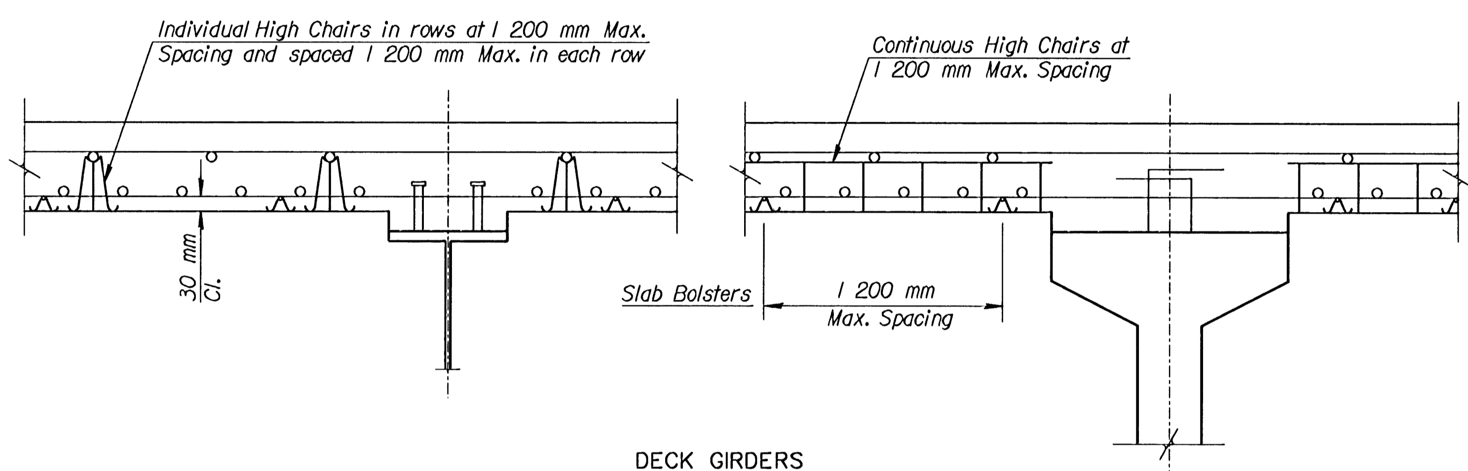
DECK GIRDERS
