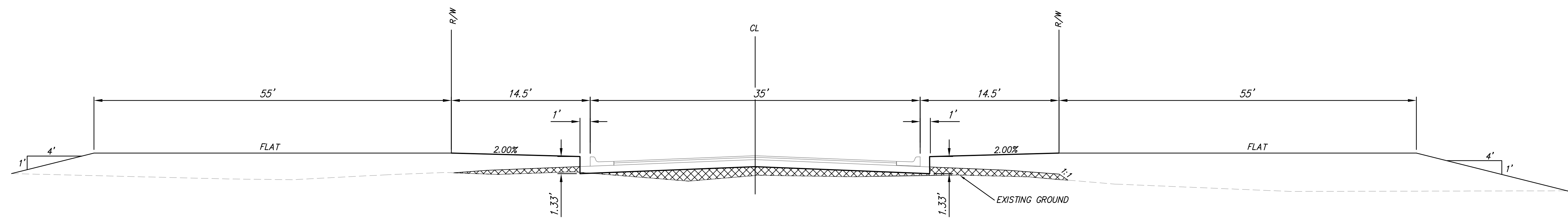
TYPICAL GRADING SECTION
