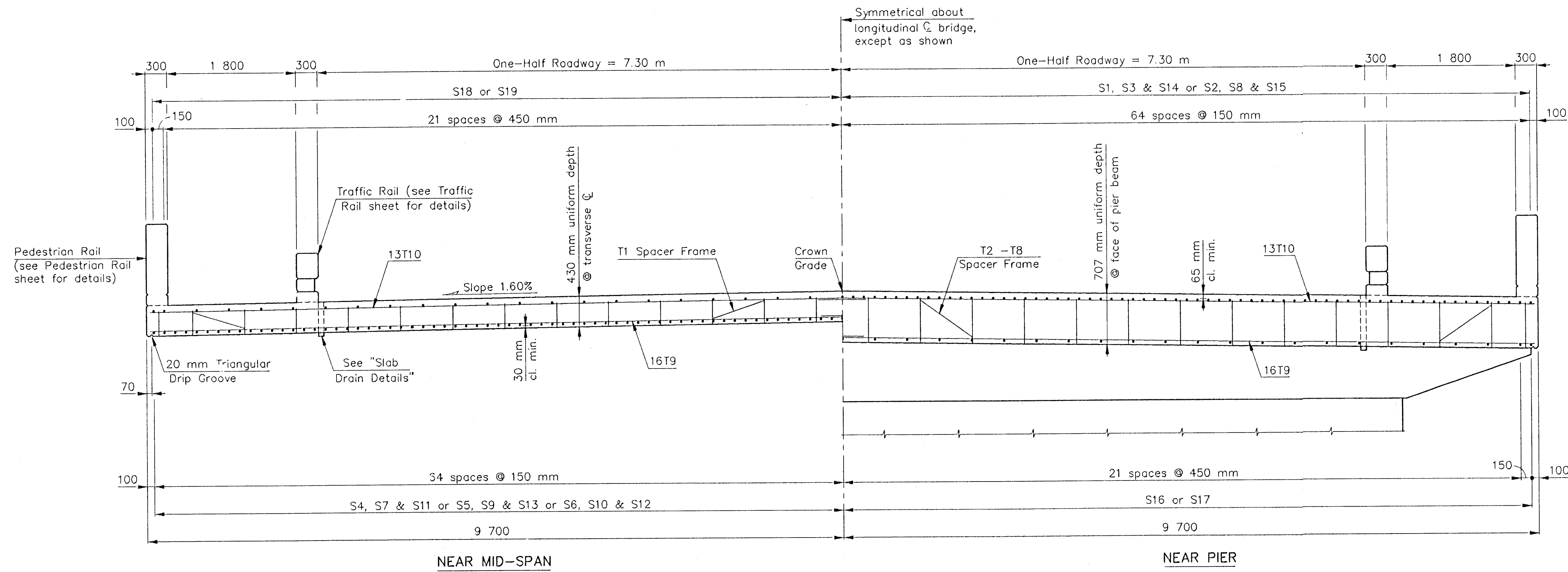
TYPICAL SECTION (Perpendicular to centerline of project)
