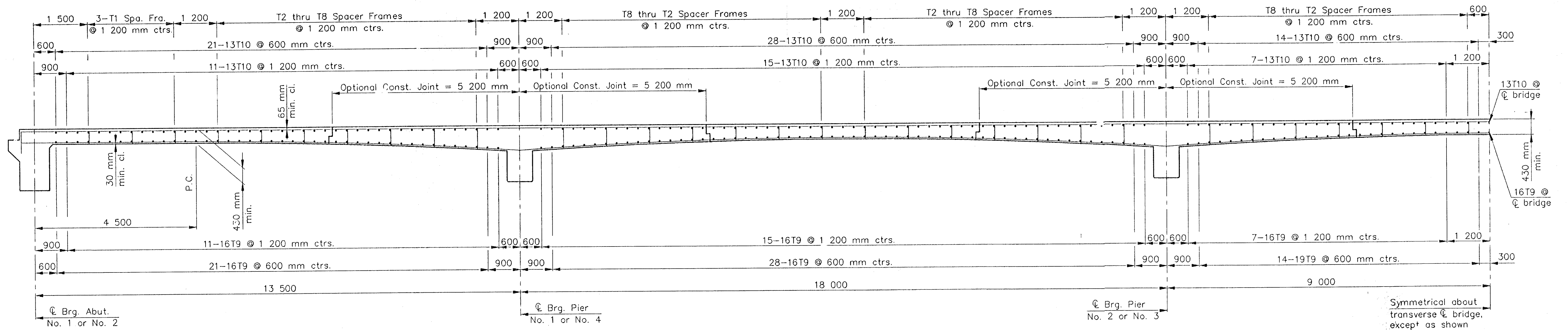
HALF LONGITUDINAL SECTION ALONG CROWN GRADE
