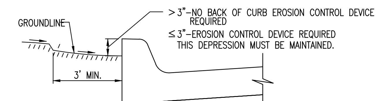
CURB BACKFILL DETAIL
