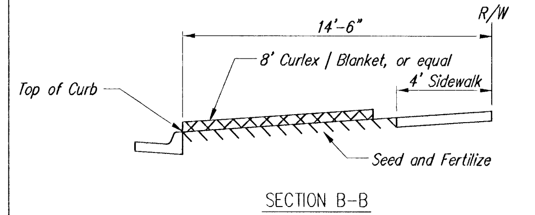
SECTION B-B
