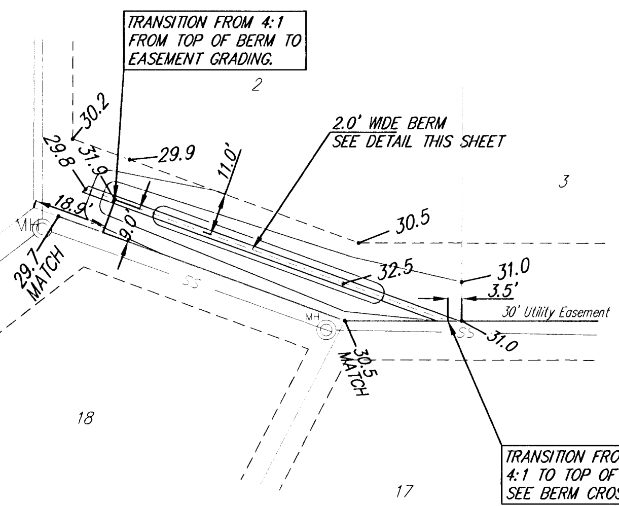
Berm Detail View
