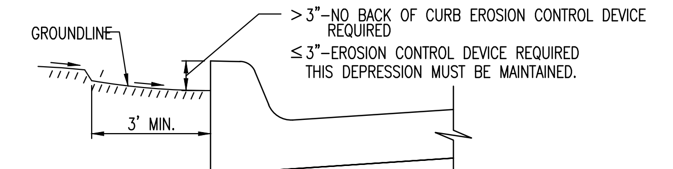
CURB BACKFILL DETAIL
