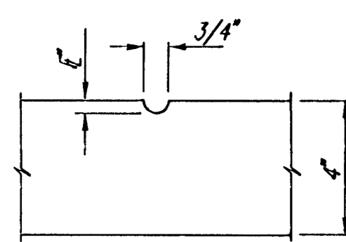
GROOVE DETAIL
