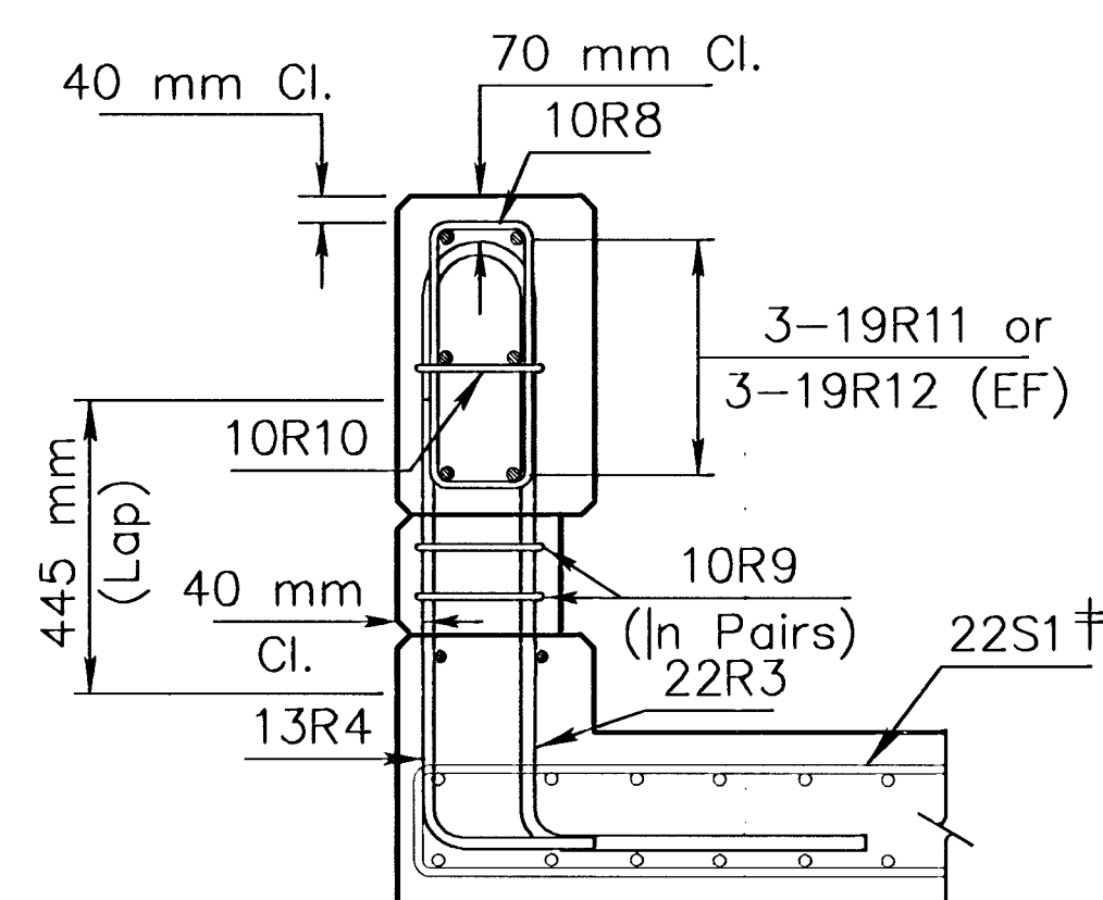
SECTION THRU INTERIOR POST
