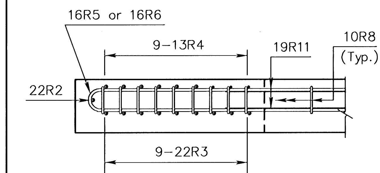
SECTION C-C
