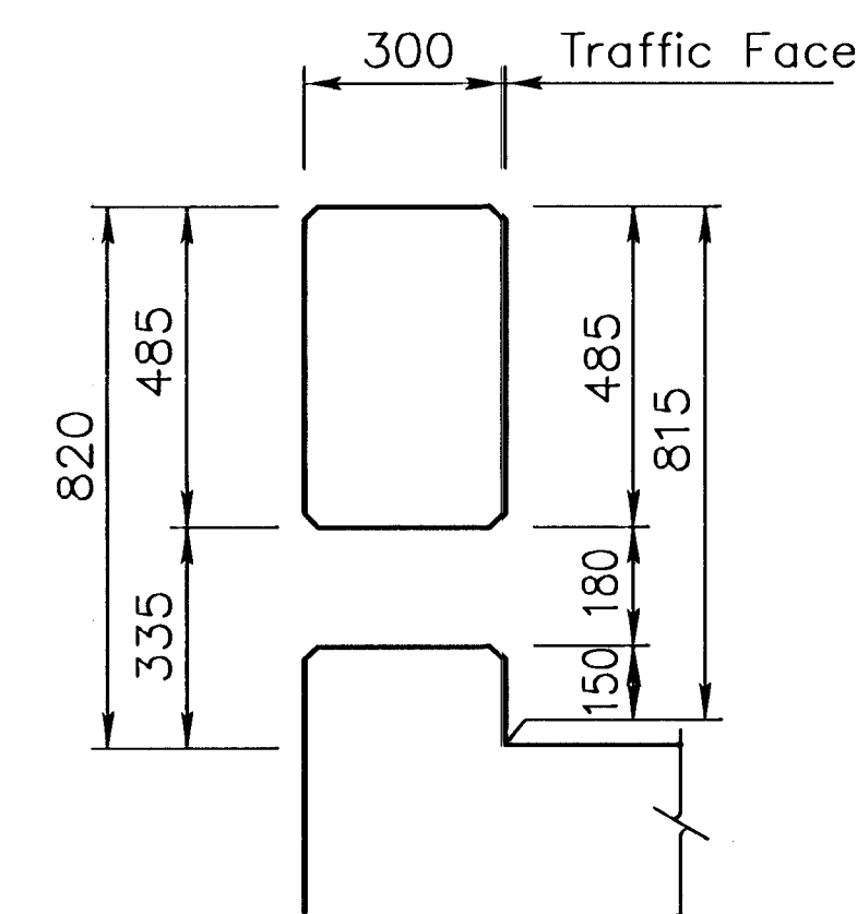
TYPICAL SECTION BETWEEN POST
