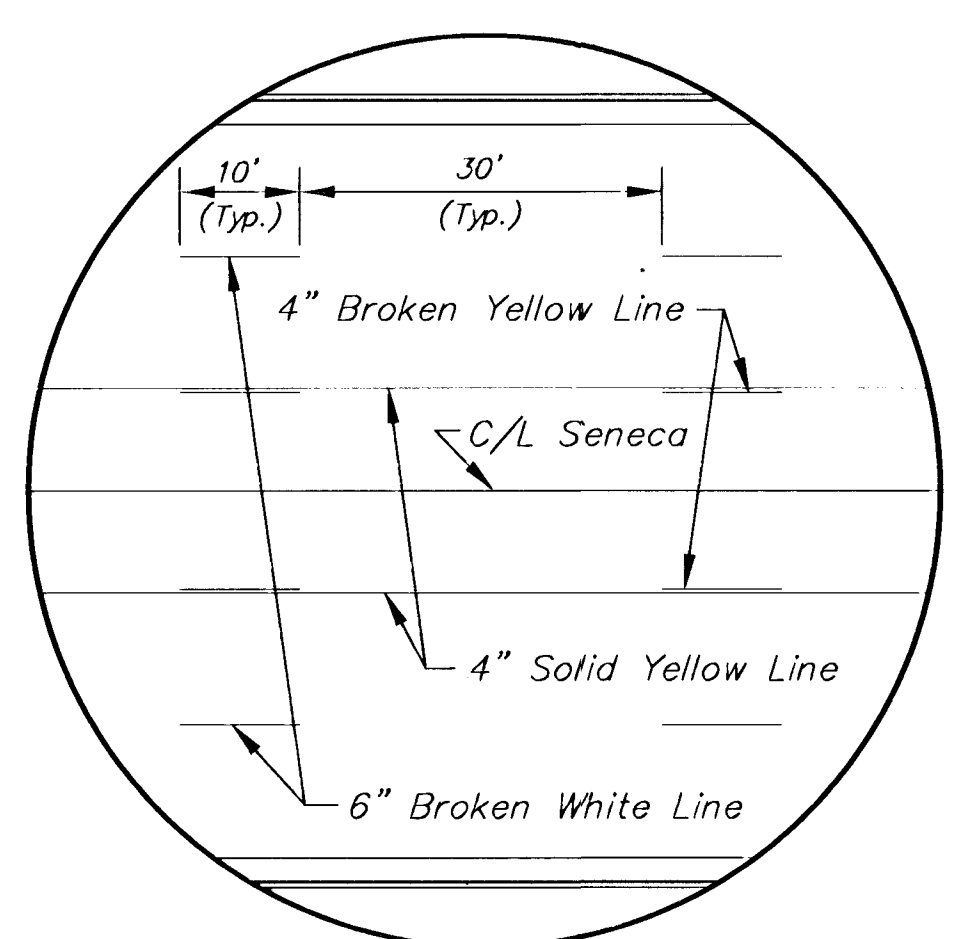
DETAIL "B"
