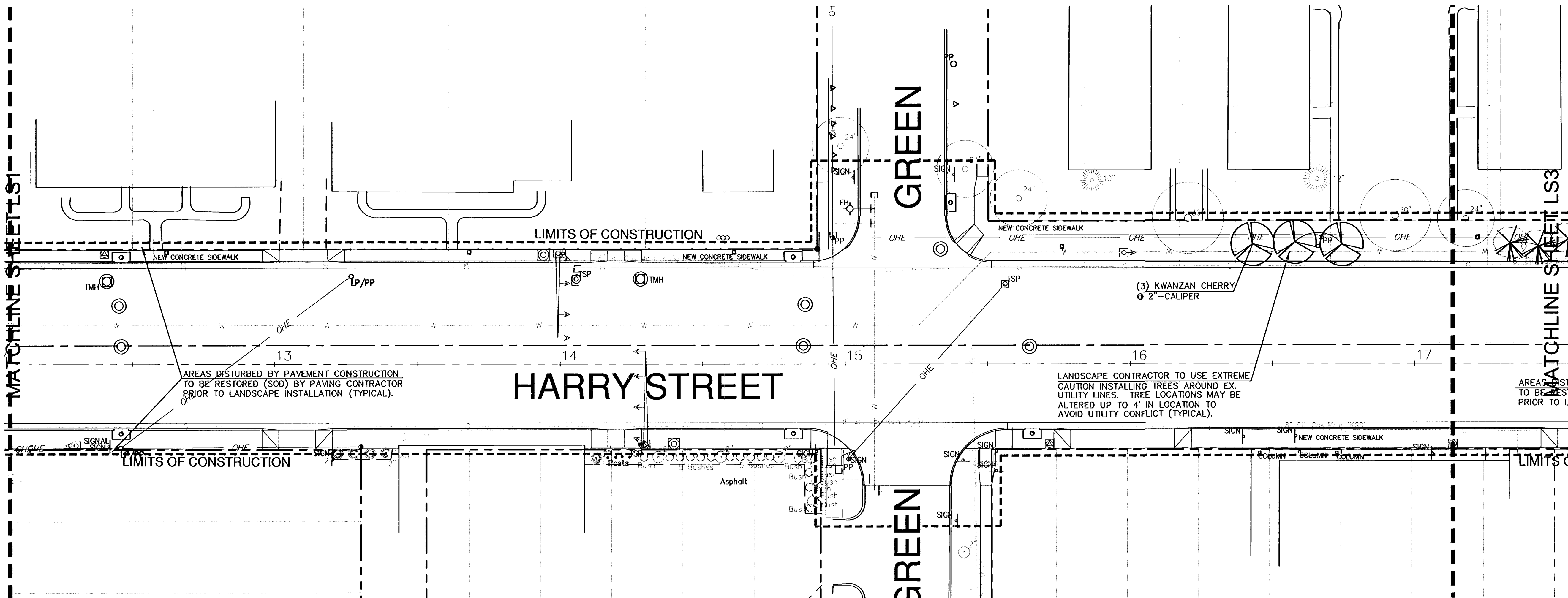
STREET PLANTING PLAN SCALE: 1"=20'-0"
