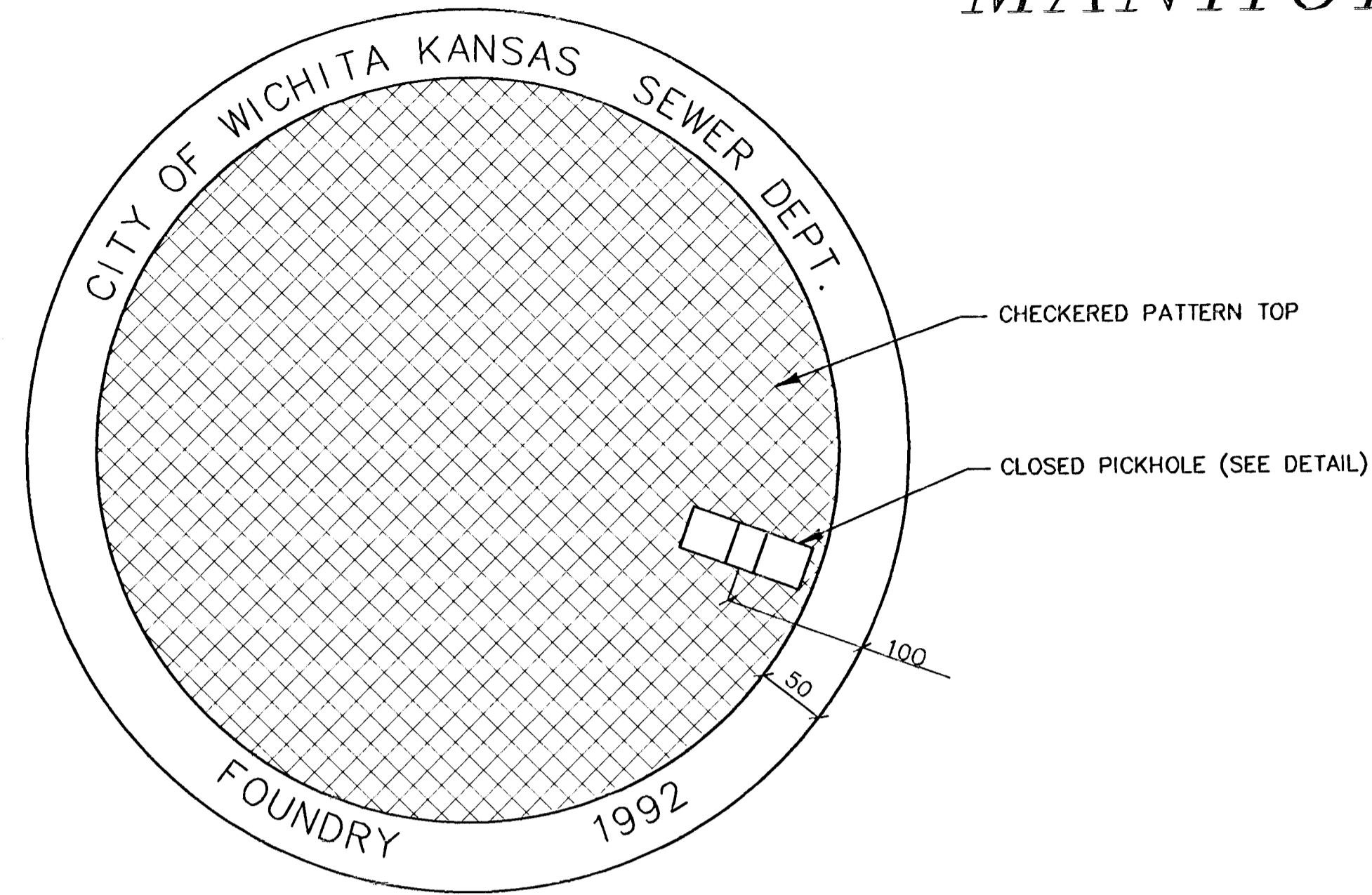
TOP VIEW
