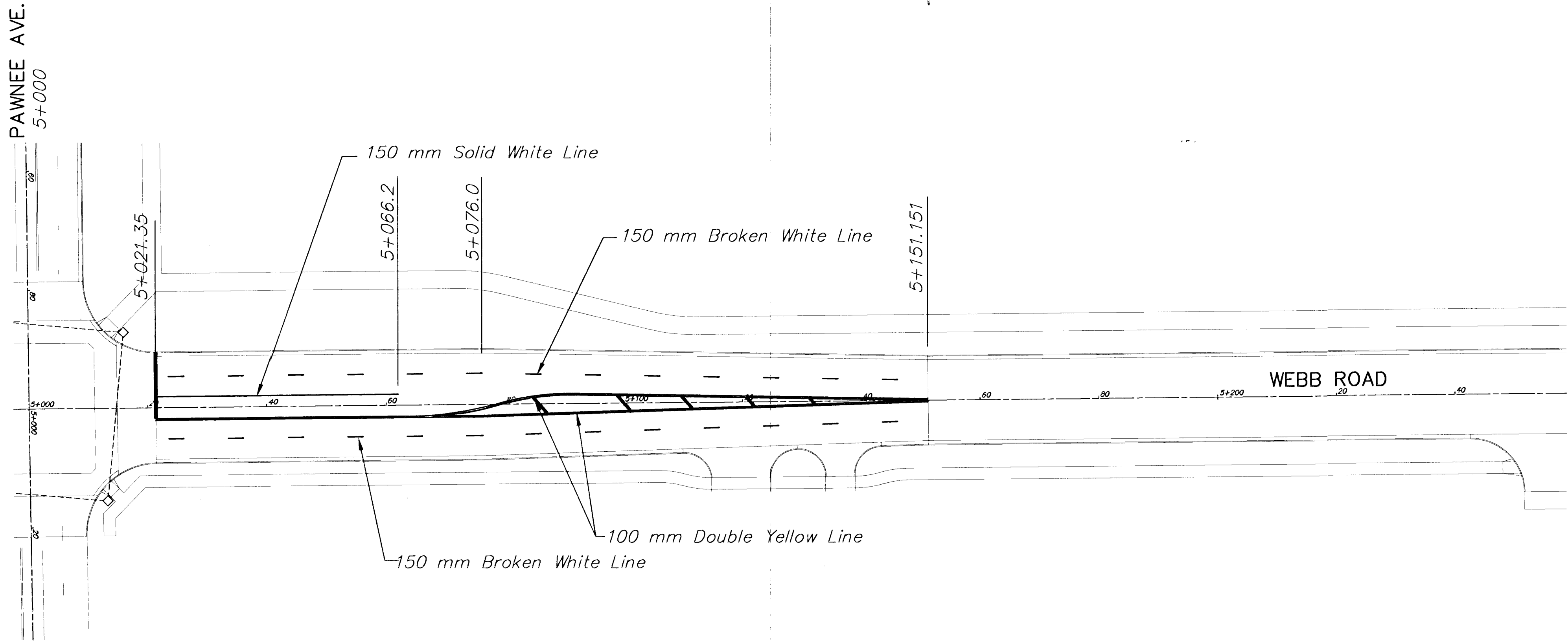
WEBB ROAD MARKING PLAN
