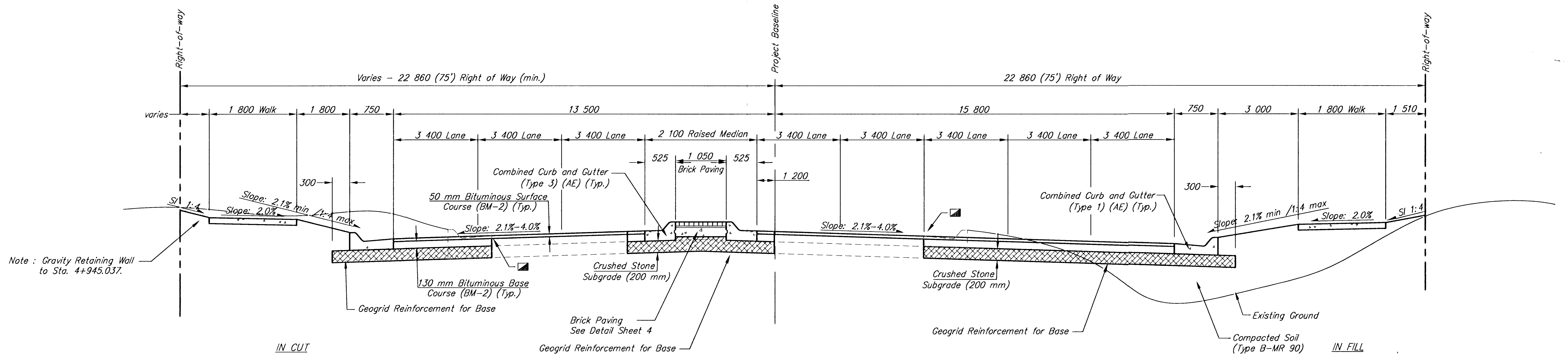
TYPICAL SECTION 4+943.902 TO 4+959.392
