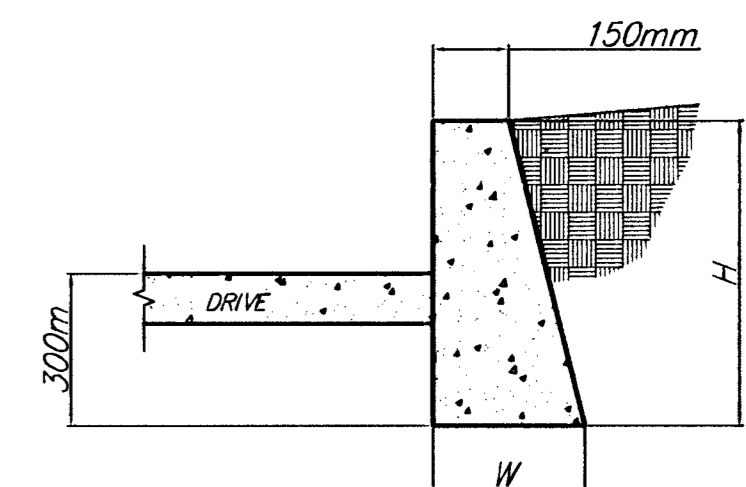
GRAVITY WALL DETAIL (CONCRETE)
