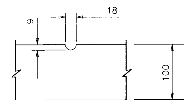
GROOVE DETAIL
