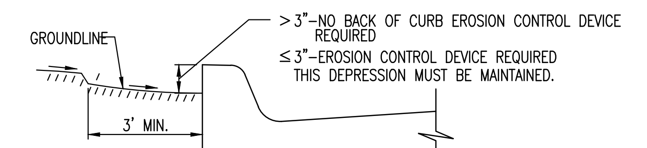
CURB BACKFILL DETAIL
