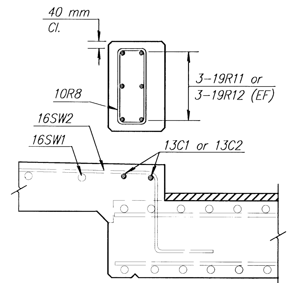
TYPICAL SECTION BETWEEN POSTS
