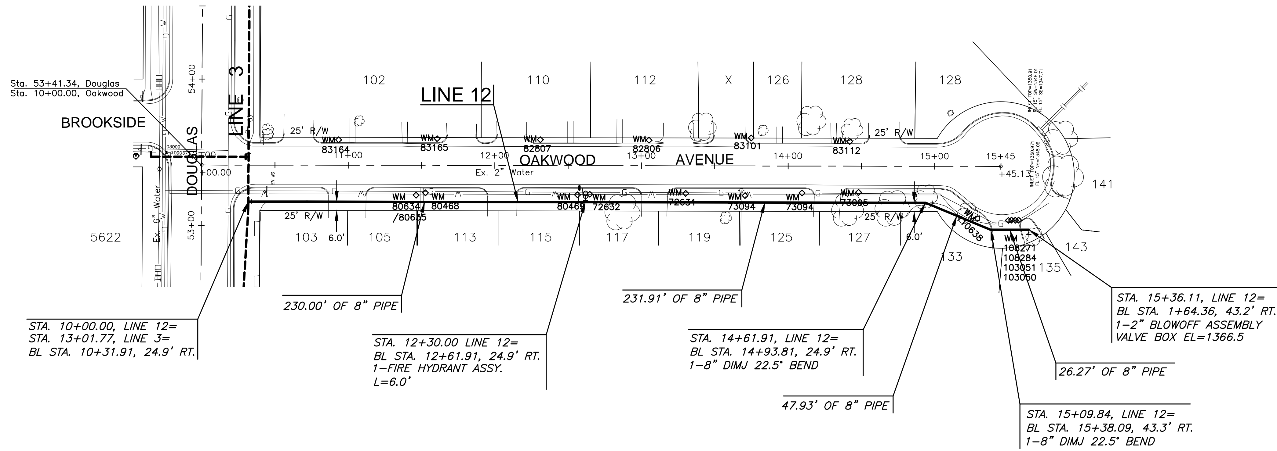
PLAN LINE 12 PROFILE LINE 12
