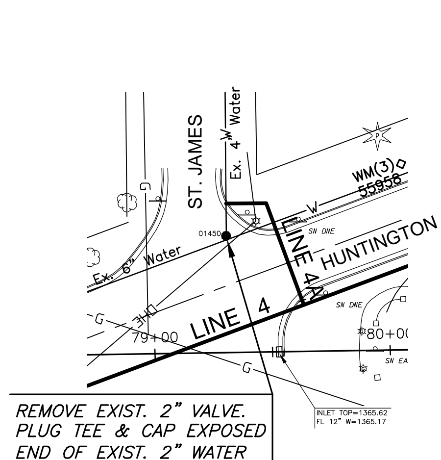
HUNTINGTON & ST. JAMES DISCONNECT #25
