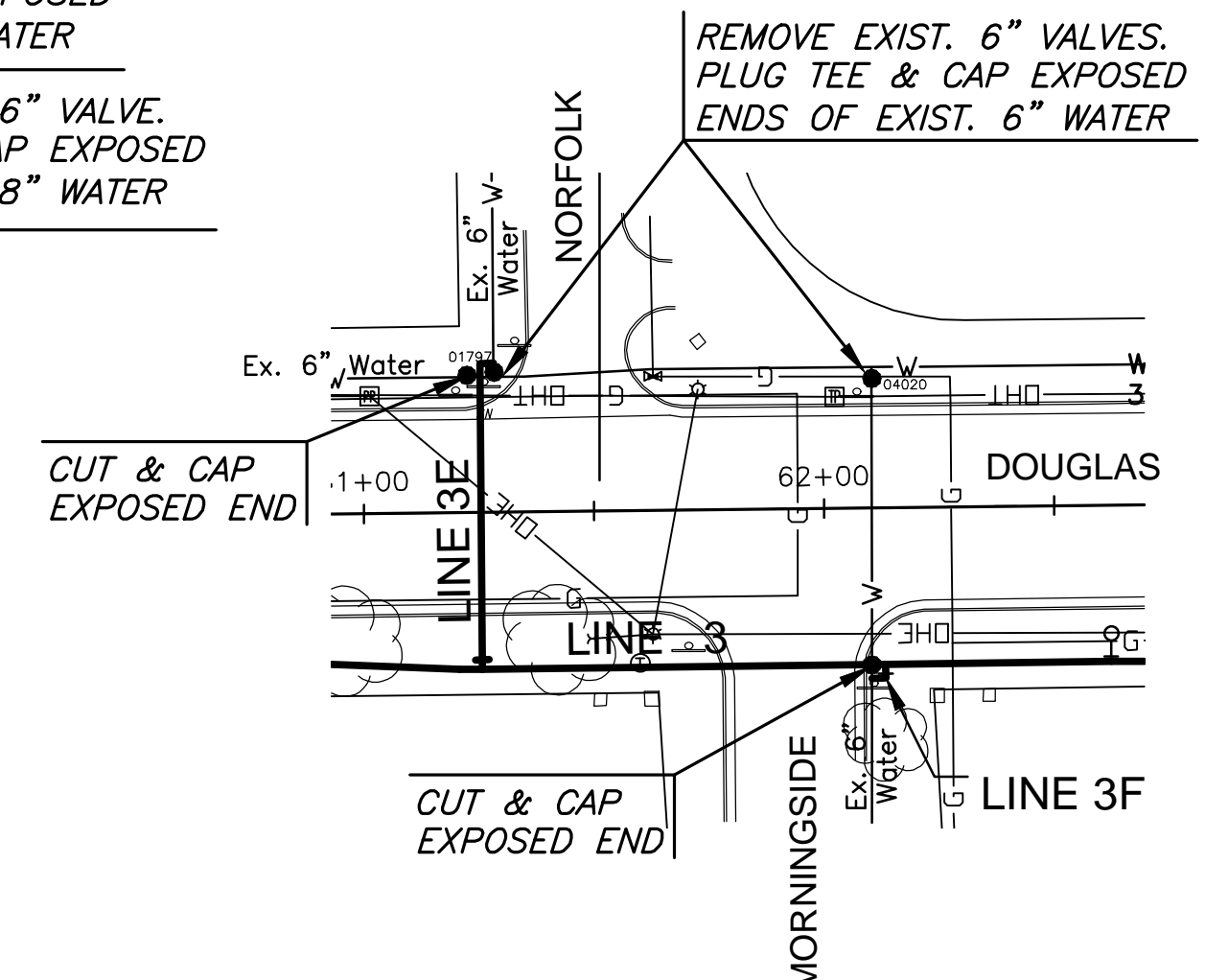
DOUGLAS & NORFOLK, MORNINGSIDE DISCONNECT #19
