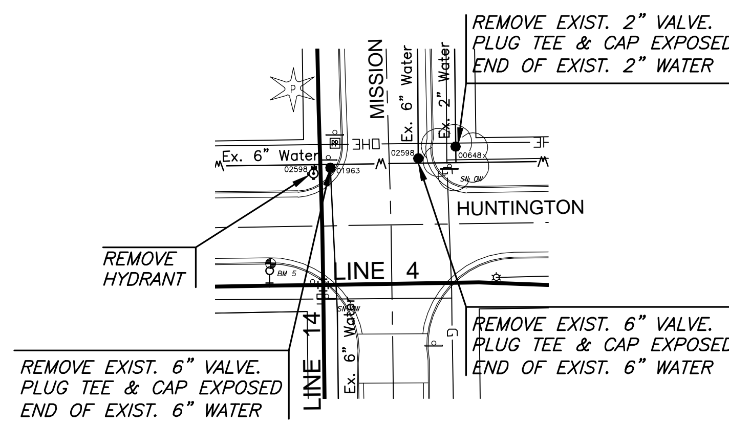
HUNTINGTON & MISSION DISCONNECT #27
