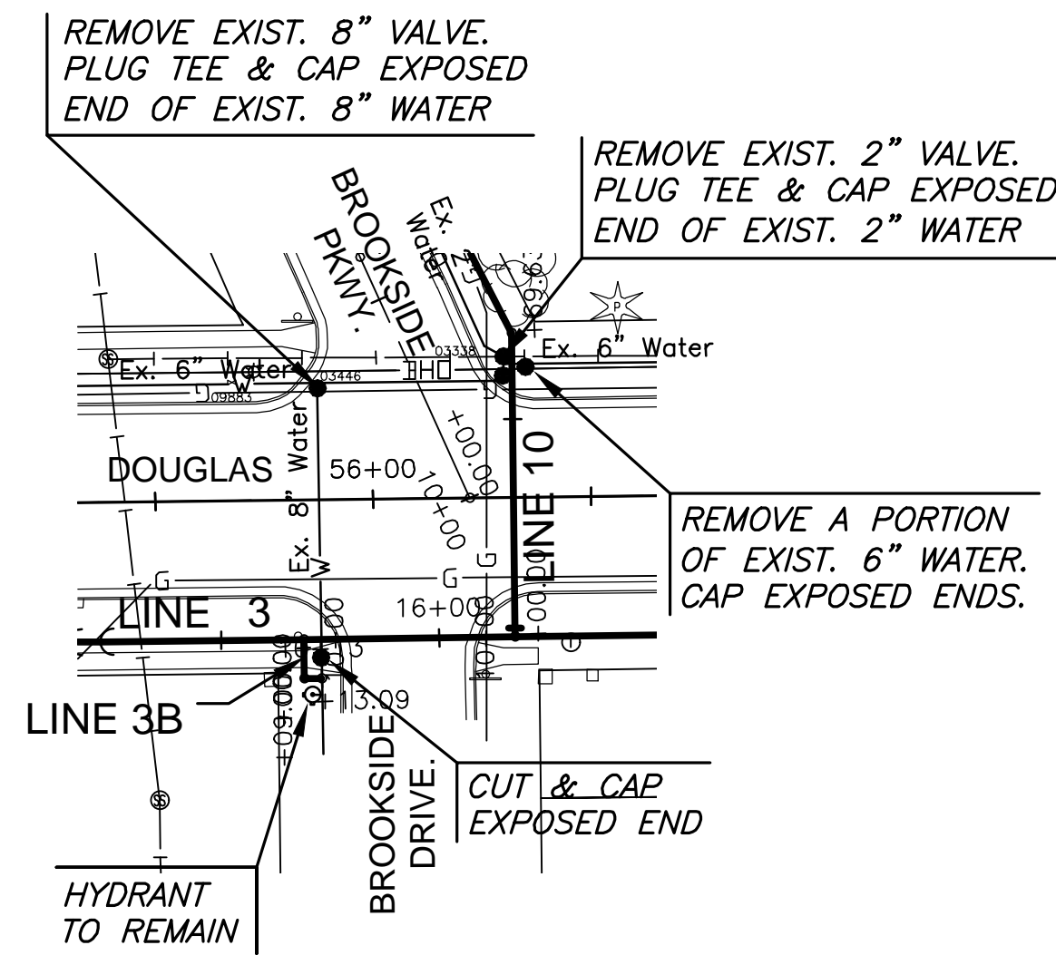
DOUGLAS & BROOKSIDE DISCONNECT #17
