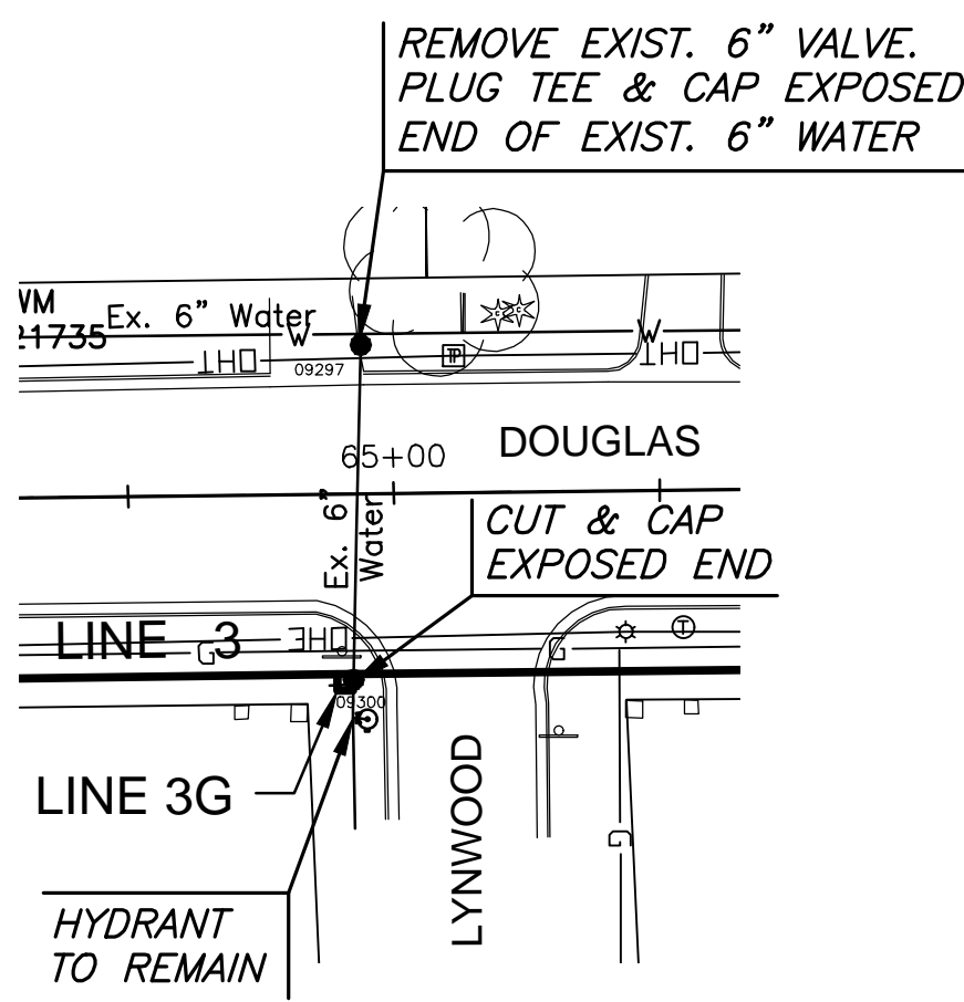
DOUGLAS & LYNWOOD DISCONNECT #20
