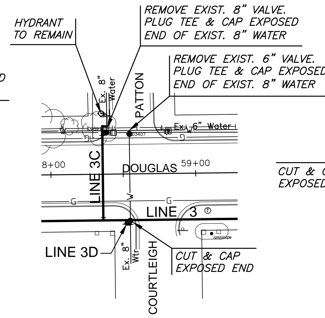
DOUGLAS & PATTON DISCONNECT #18
