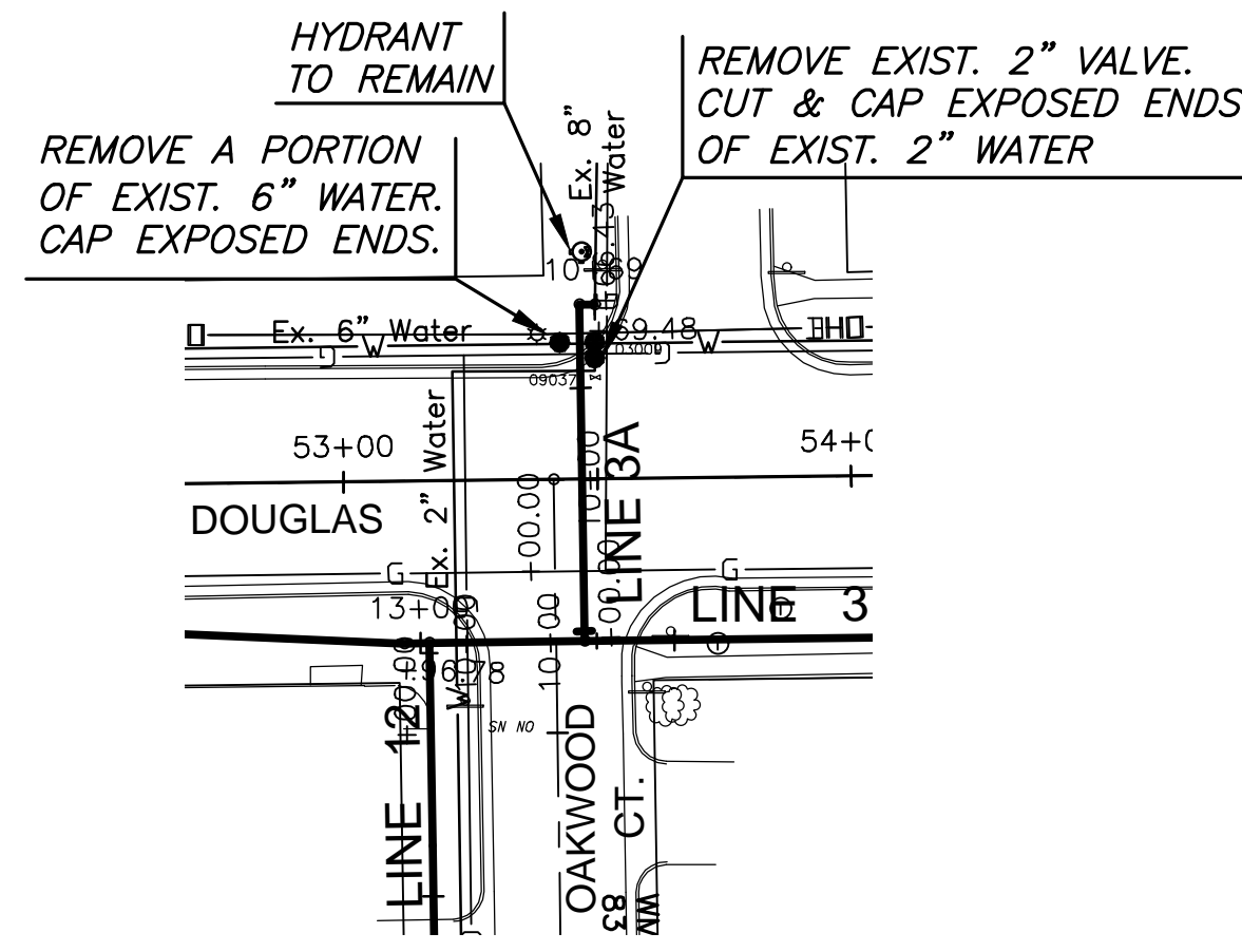
DOUGLAS & OAKWOOD CT. DISCONNECT #16
