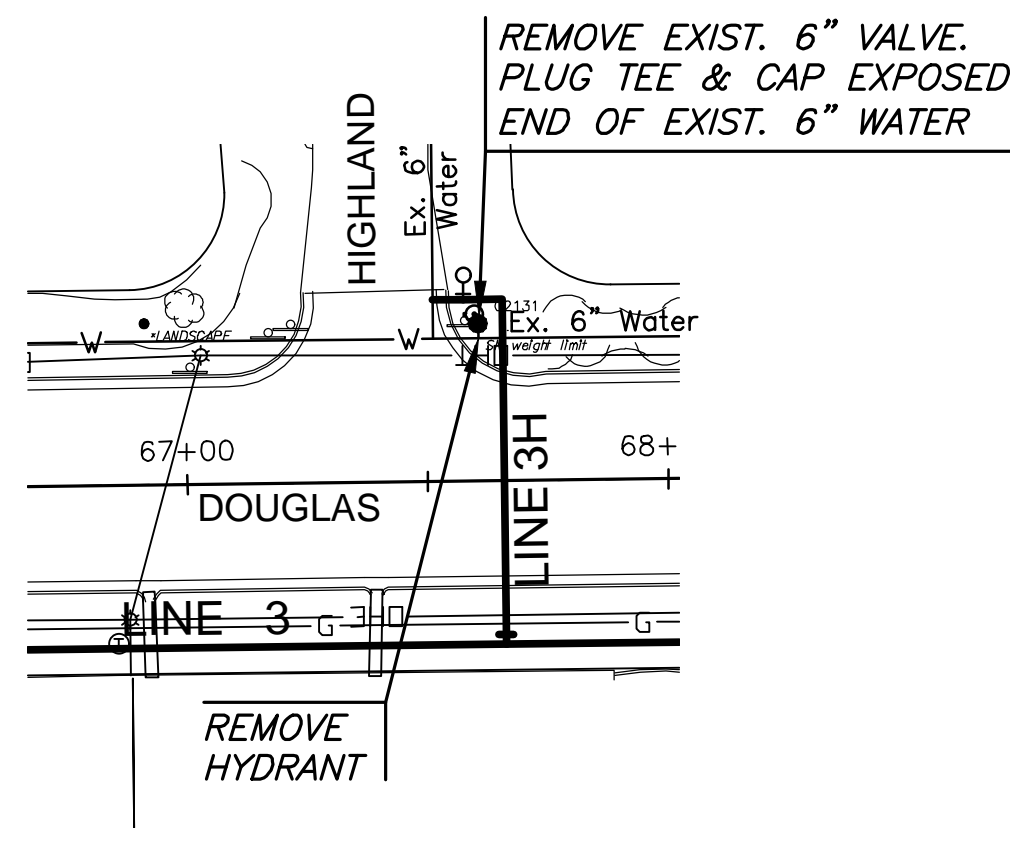
DOUGLAS & HIGHLAND DISCONNECT #21
