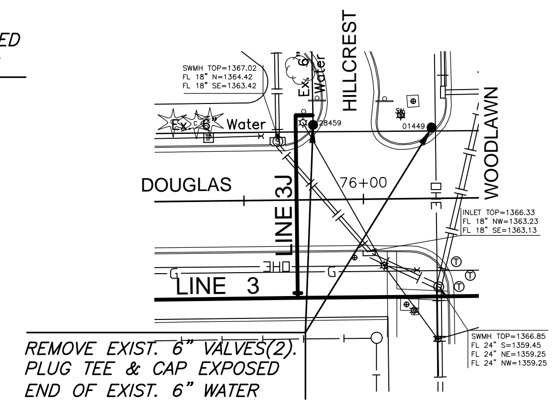
DOUGLAS & HILLCREST DISCONNECT #24
