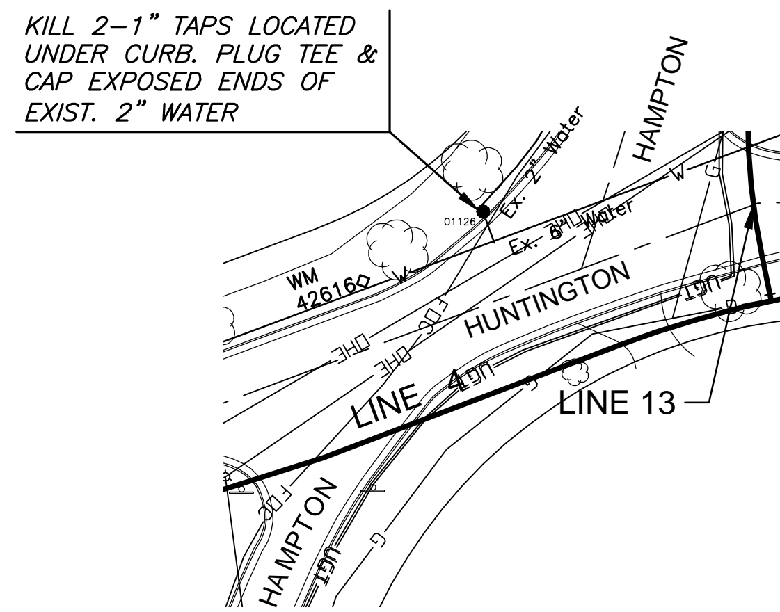
HUNTINGTON & HAMPTON DISCONNECT #26
