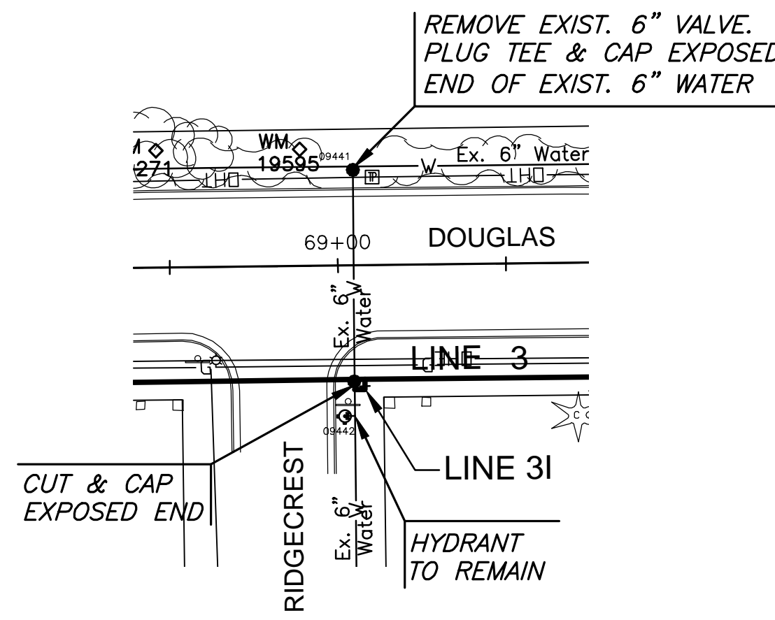
DOUGLAS & RIDGCREST DISCONNECT #22
