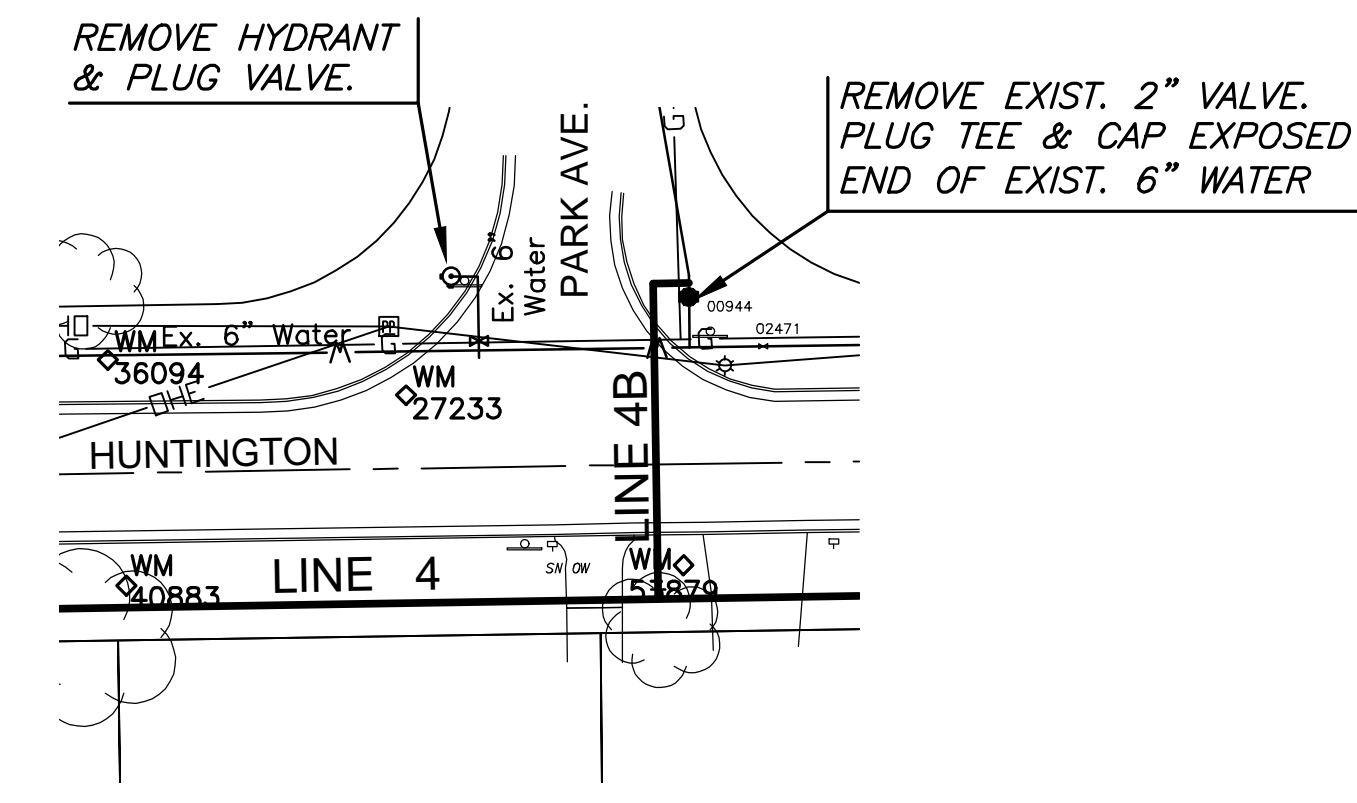
HUNTINGTON & PARK AVE DISCONNECT #28
