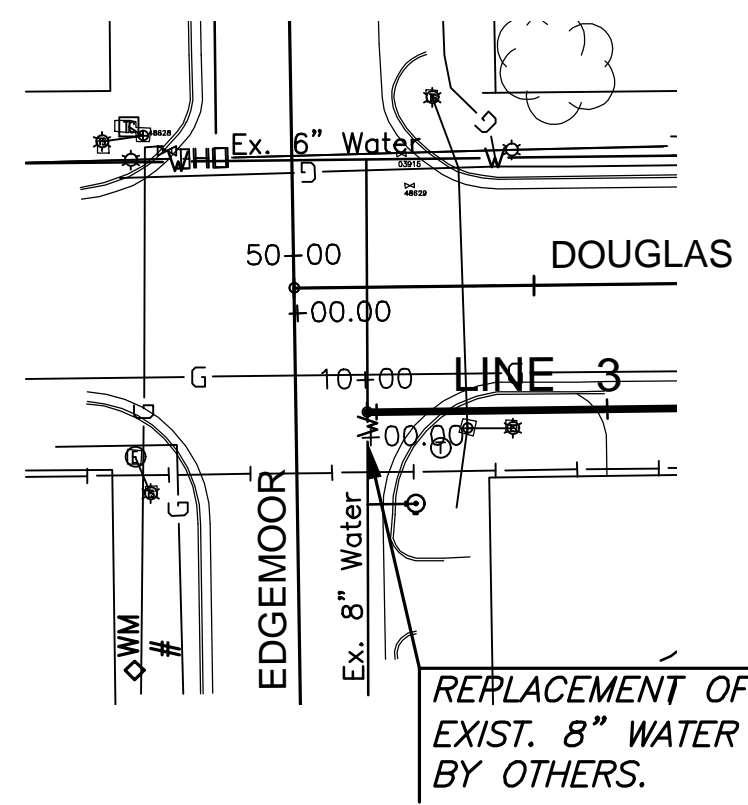
DOUGLAS & EDGEMOOR DISCONNECT #15
