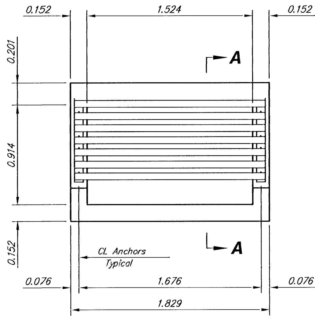
END VIEW
