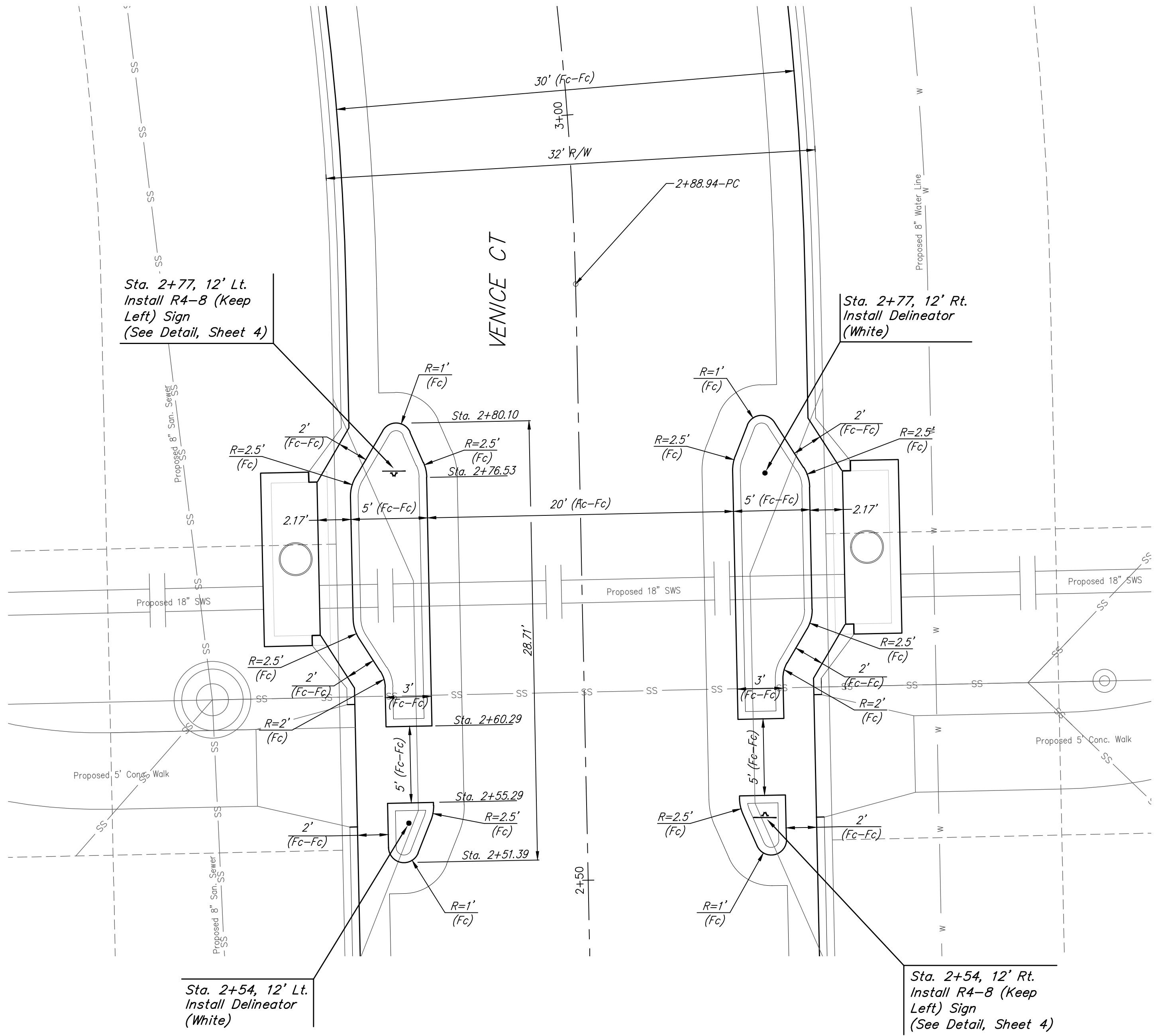
CHICANE DETAIL Geometric Dimensions
