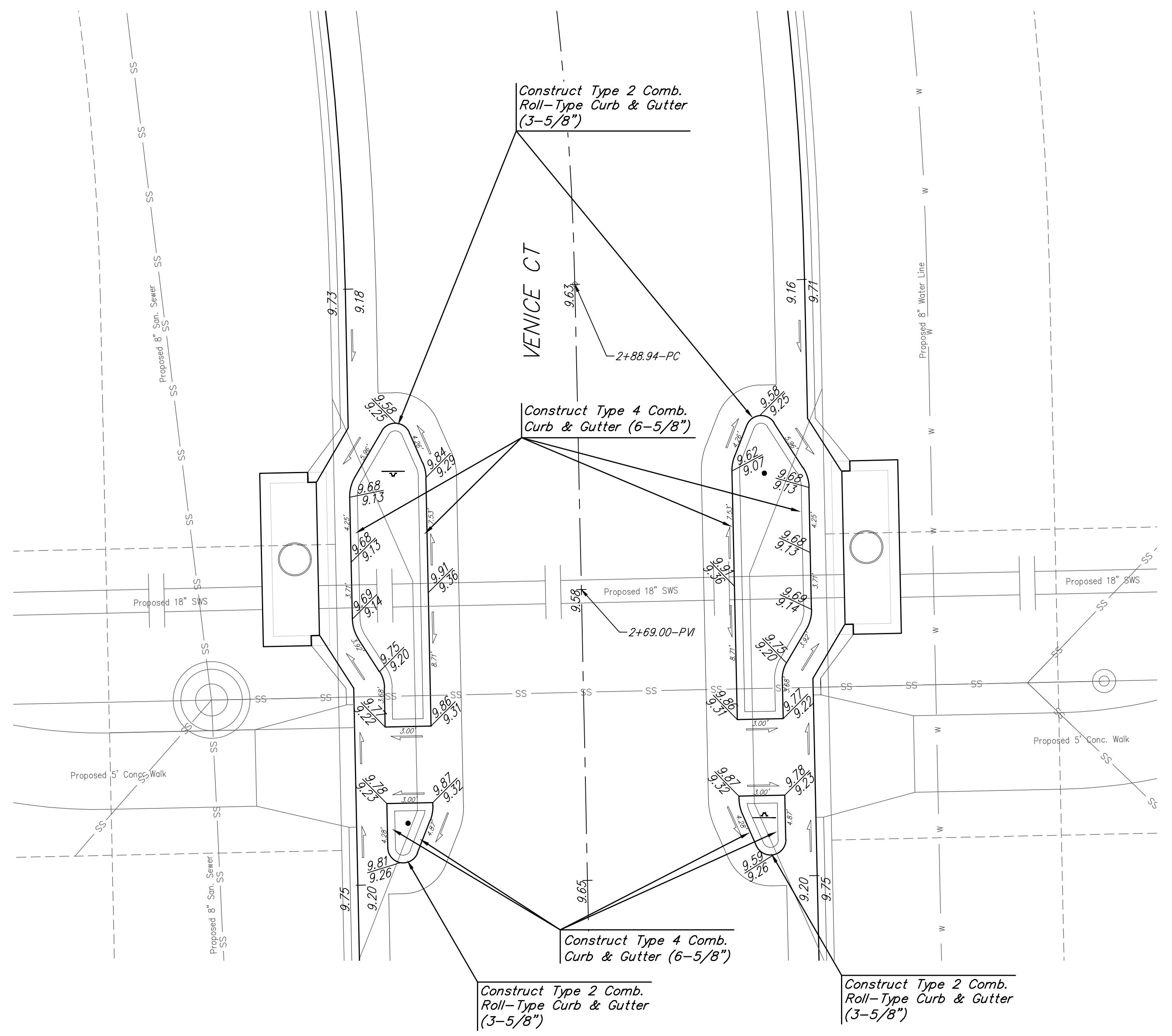
CHICANE DETAIL Elevation Plan
