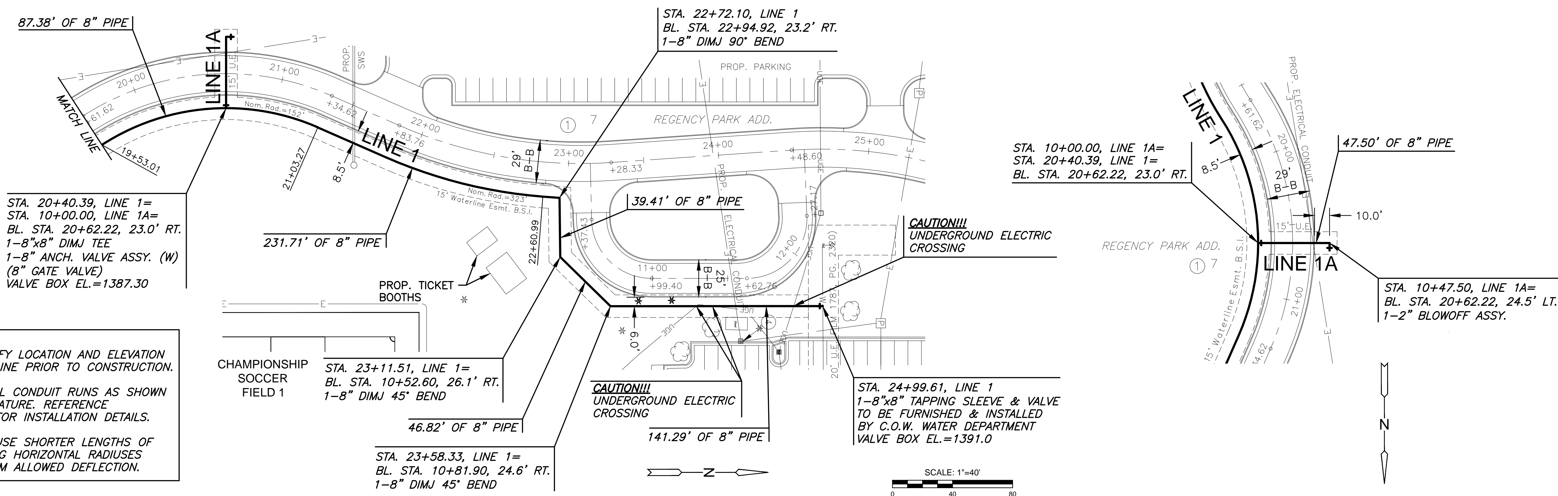
PLAN WATER LINE 1 (CONT.) PROFILE WATER LINE 1 (CONT.)
